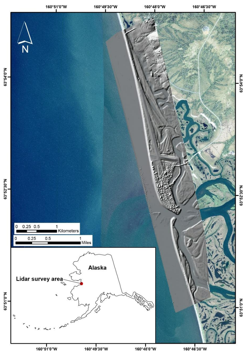
FIGURE 1. Location map of 2005 LiDAR data collection area over the coastal community of Unalakleet, Alaska, and displayed as a hillshaded raster overlain on 2005 IKONOS-2 satellite imagery.
