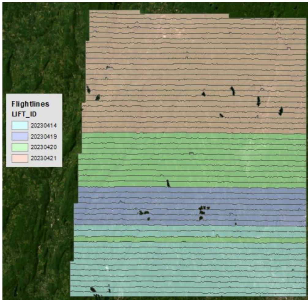
Figure 3. Delivery Block 01 swaths
