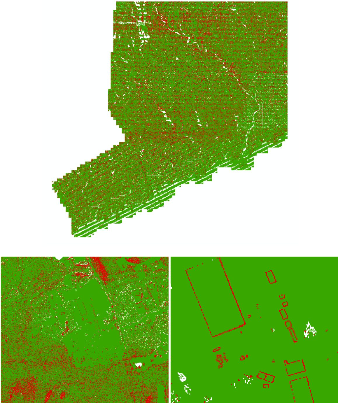
Figure 6. Intra-swath relative accuracy. The top image shows the full project area; areas where the maximum difference is \leq 6 cm per pixel within each swath are colored green and areas exceeding 6 cm are colored red. The left image shows a large portion of the dataset; flat, open areas are colored green as they are within 6 cm whereas sloped terrain is colored red because it exceeds 6 cm maximum difference, as expected, due to
