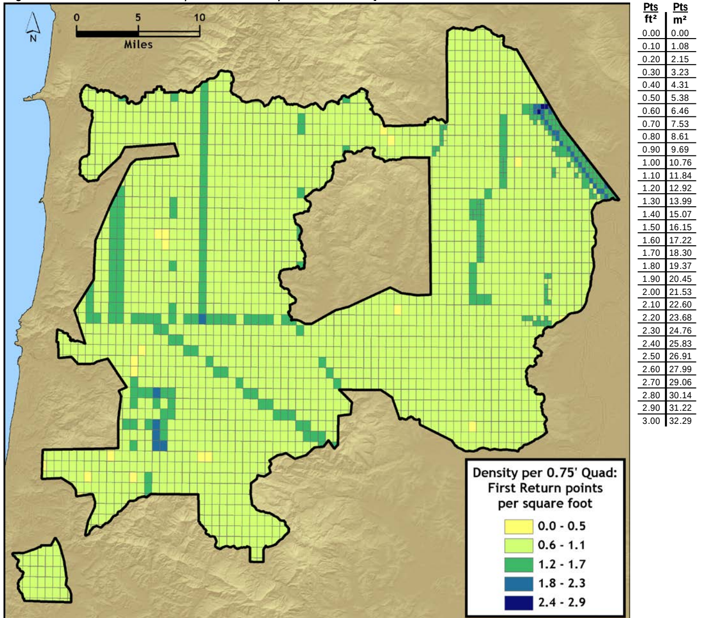
Figure 4.2. First return laser point densities per 0.75' USGS Quad for data delivered to date.
