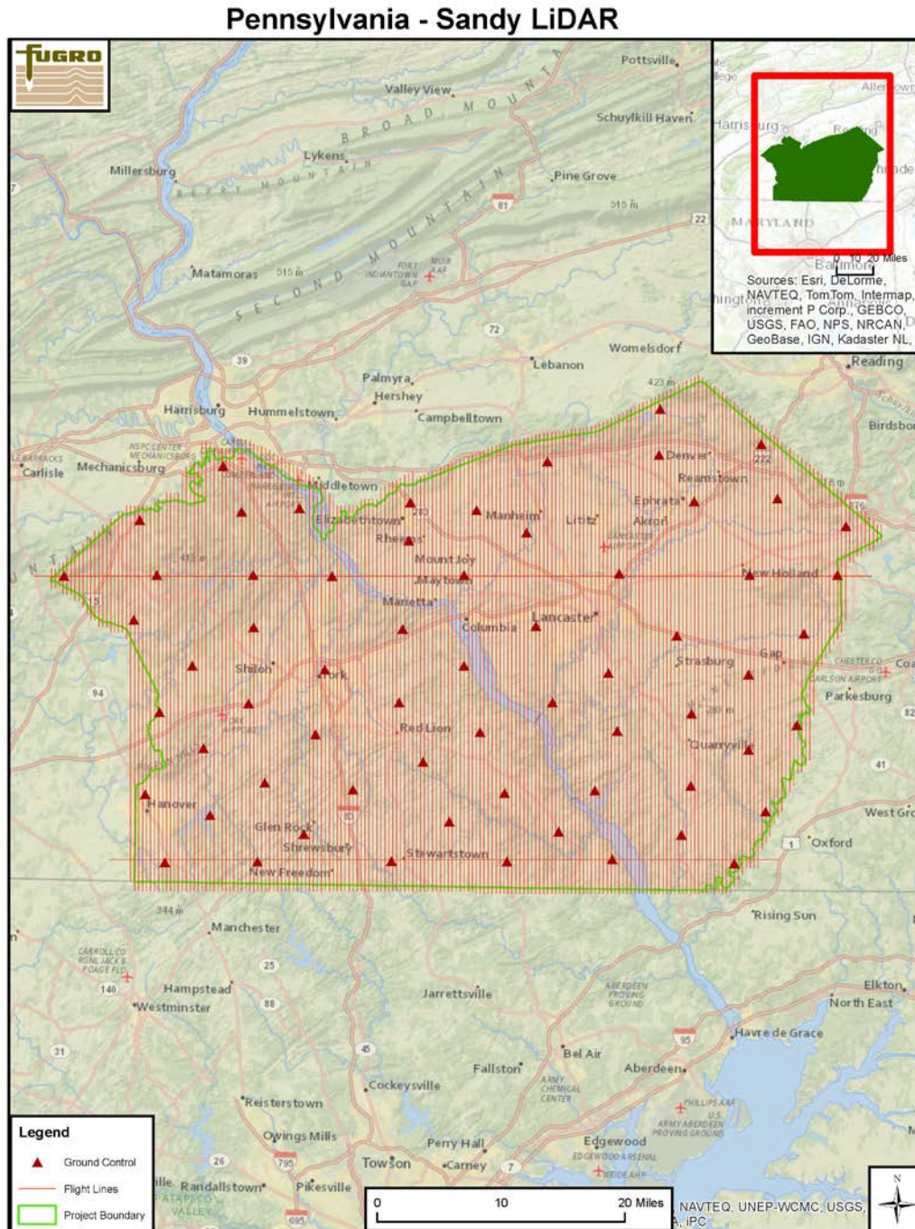
Figure 3: Planned Flight Diagram
