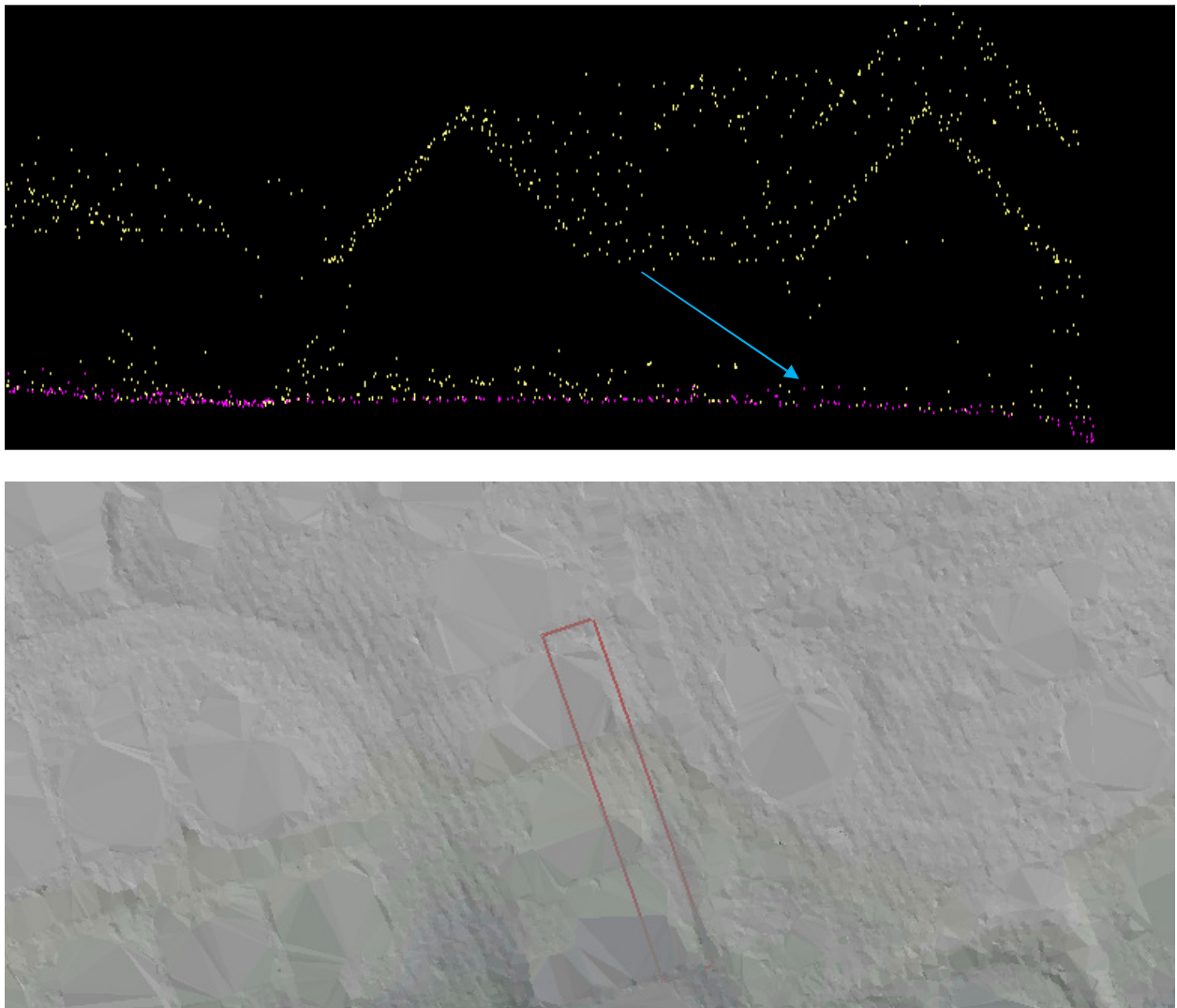
Figure 6 – Tile number 6121-01. Profile with points colored by class (class 1=yellow, class 2=pink) is shown in the top view and a TIN of the surface is shown in the bottom view. The arrow identifies low vegetation points. A limited number of these small features are still classified as ground but do not impact the usability of the dataset.
