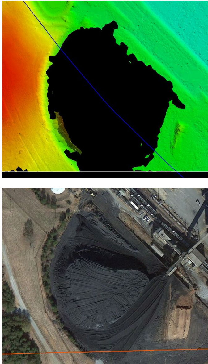
Figure 10 – Tile 5061-04. Top: TIN model showing large void over a coal field right along the project boundary (blue outline). The dark colored attribute of the coal absorbs LiDAR and does not provide many useable returns. Bottom: Aerial showing the processing facility.
