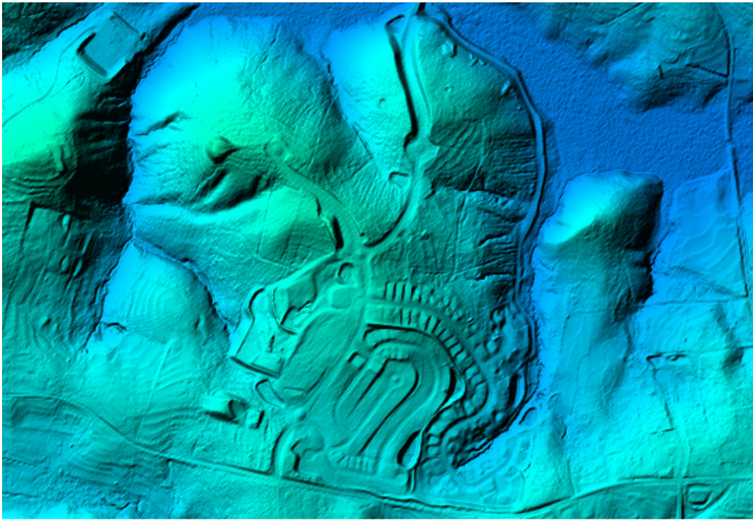
Figure 12 – An example of the bare earth DEM.
