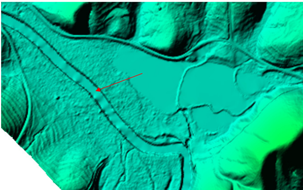
Figure 13 - The bare earth DEM showing water artifacts within a river breakline.
