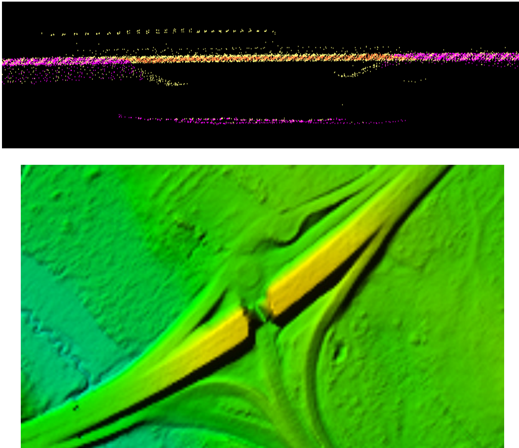
Figure 7 – The DEM in the bottom view shows a visual artifact because the surface model is interpolated from the ground points on the slope leading to the bridge to the lower ground points on either side of the bridge. The surface model must make a continuous model and in order to do so, points are connected through interpolation. This can cause visual artifacts when there are features with large elevation differences. The profile in the top view shows the LiDAR points of this particular feature colored by class. All bridge points have been removed from ground (pink) and are either unclassified (yellow) or bridge (orange). There are no ground points that can be modified to correct this visual artifact.
