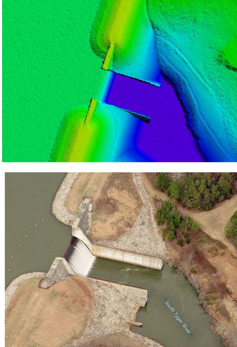
Figure 9 – Tile 6115-03. Top: TIN model showing dam remaining the final ground model. Bottom: Aerial profile view of the same location.
