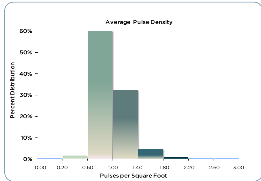
Figure 6.1. Histogram of first return laser point density for data delivered to date.
