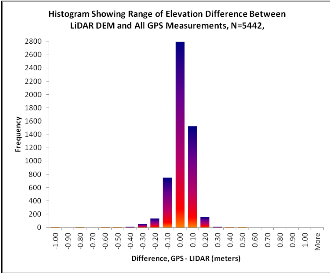
Figure 9. Histogram of Consolidated Vertical Accuracy Distribution.
