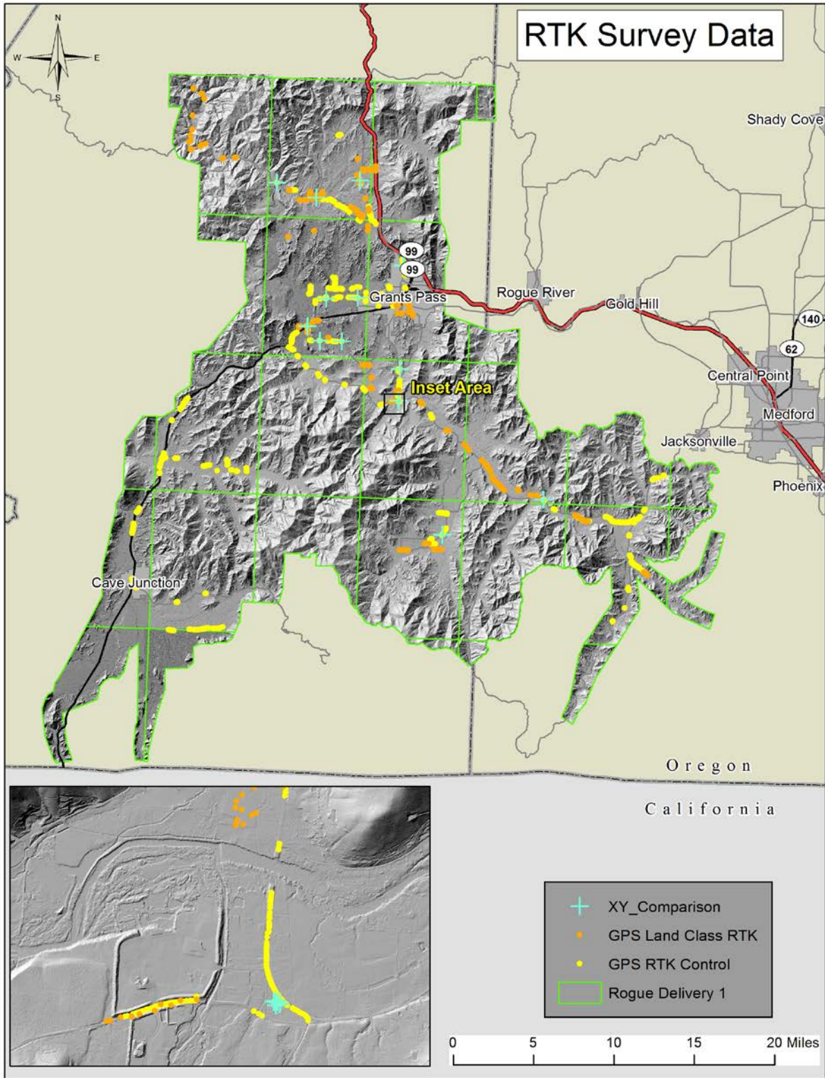
Figure 8. Locations of GPS points used in horizontal accuracy analysis.
