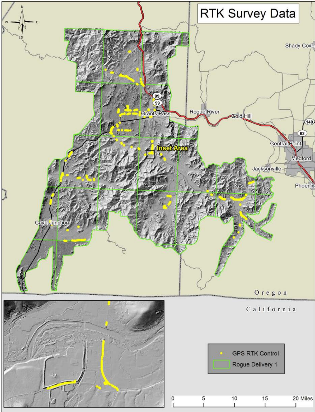
Figure 6. Locations of RTK control surveyed by DOGAMI. Data was used to test absolute accuracy for the Rogue River lidar survey within the Delivery 1 extent.
