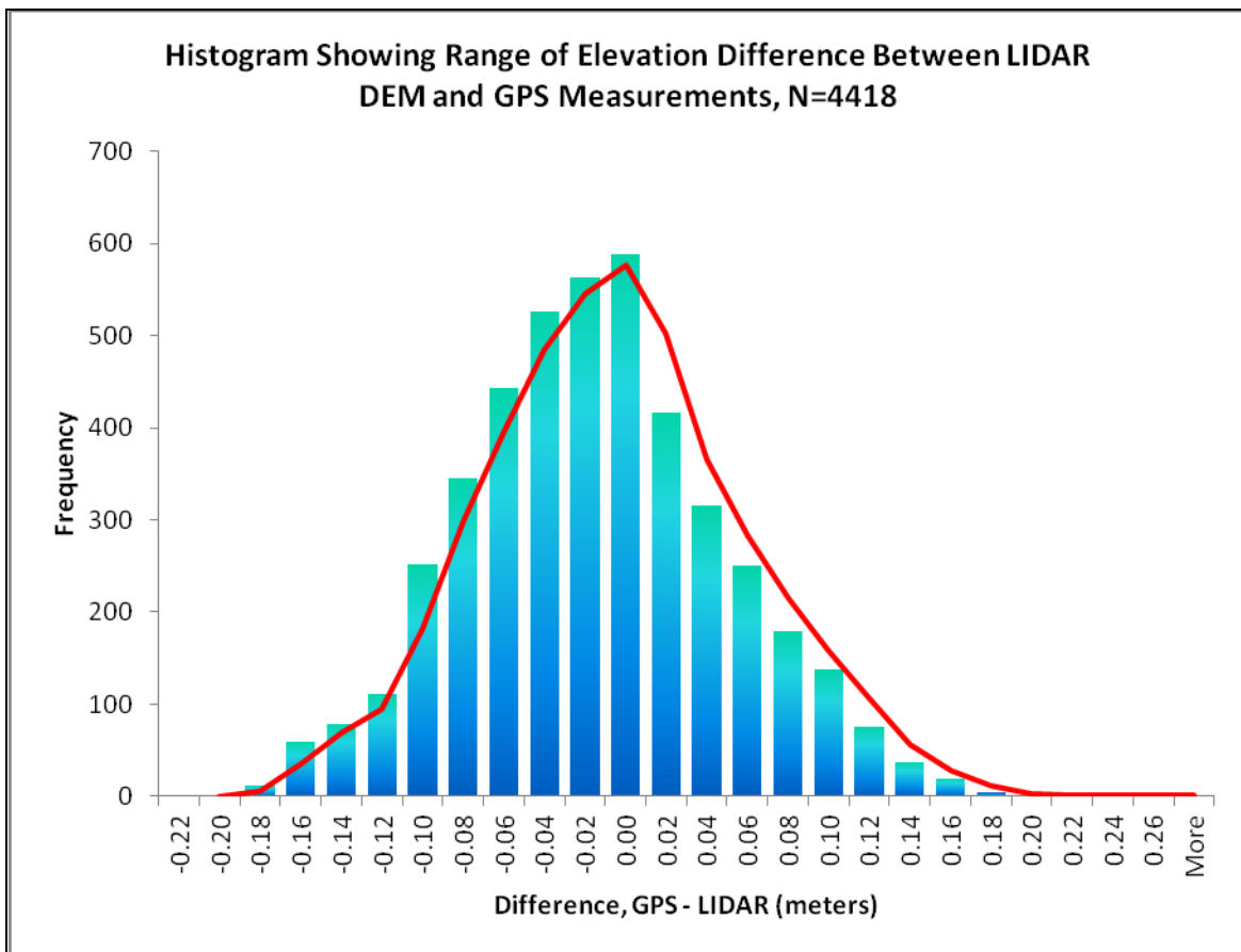
Figure 7. Histogram of absolute vertical accuracy
