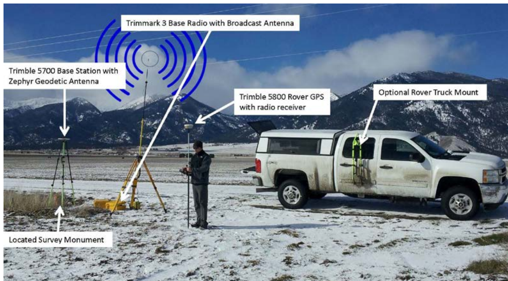
Figure 5. The Trimble 5700 base station antenna located over a known reference point at Cove, OR. Corrected GPS position and elevation information is then transmitted by a Trimmark III base radio to the 5800 GPS rover unit.
