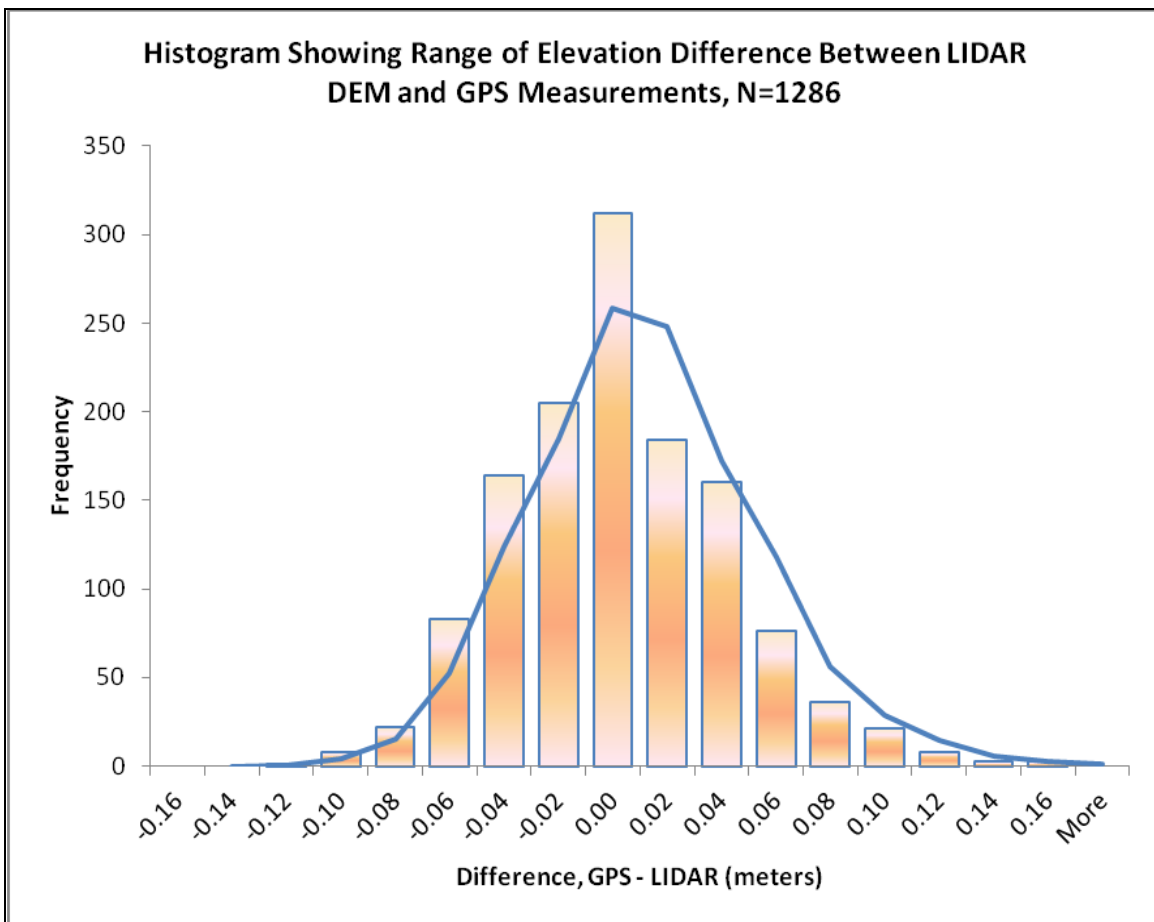
Figure 7. Histogram of absolute vertical accuracy
