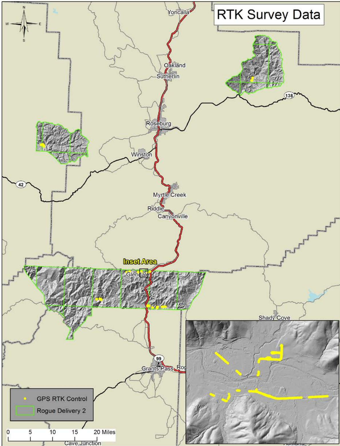
Figure 6. Locations of RTK control surveyed by DOGAMI. Data was used to test absolute accuracy for the Rogue River lidar survey within the Delivery 2 extent.
