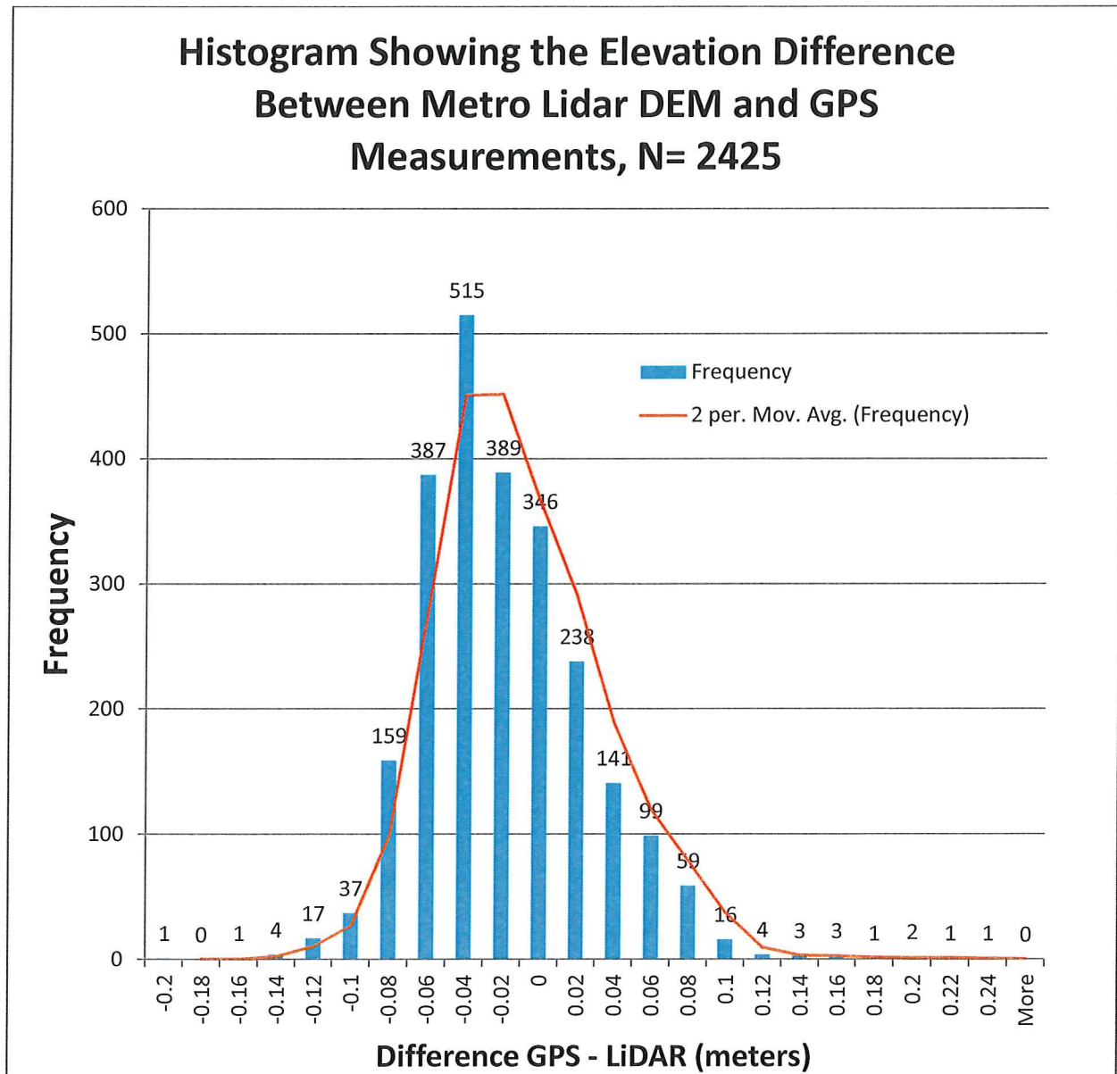
Figure 12. Histogram of absolute vertical accuracy in meters.
