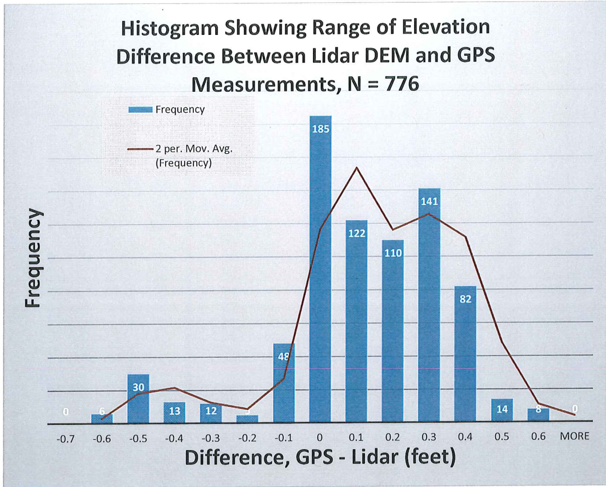
Figure 13. Histogram of absolute vertical accuracy in feet.
