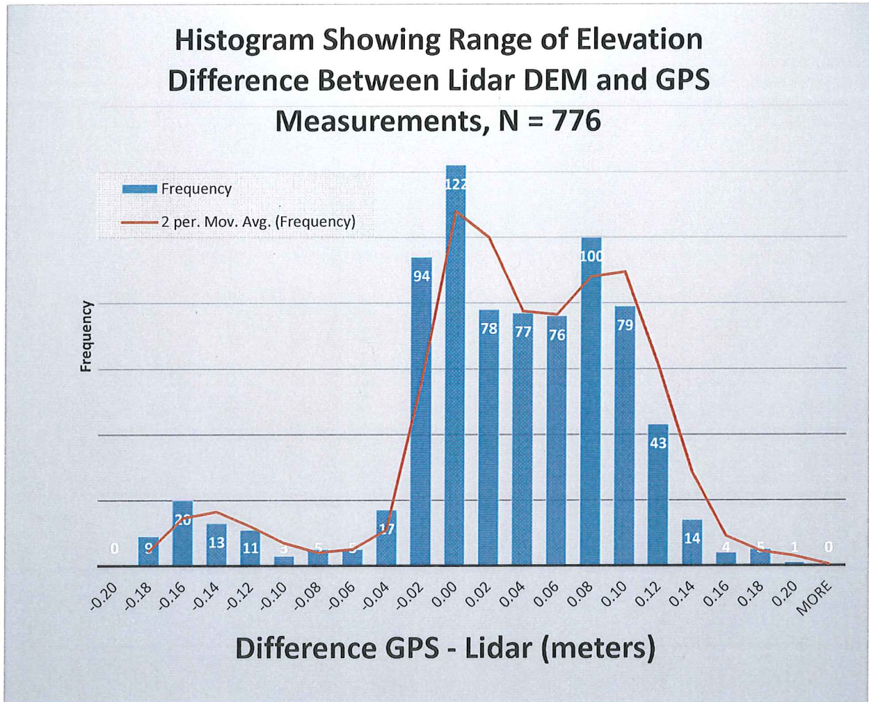
Figure 12. Histogram of absolute vertical accuracy in meters.
