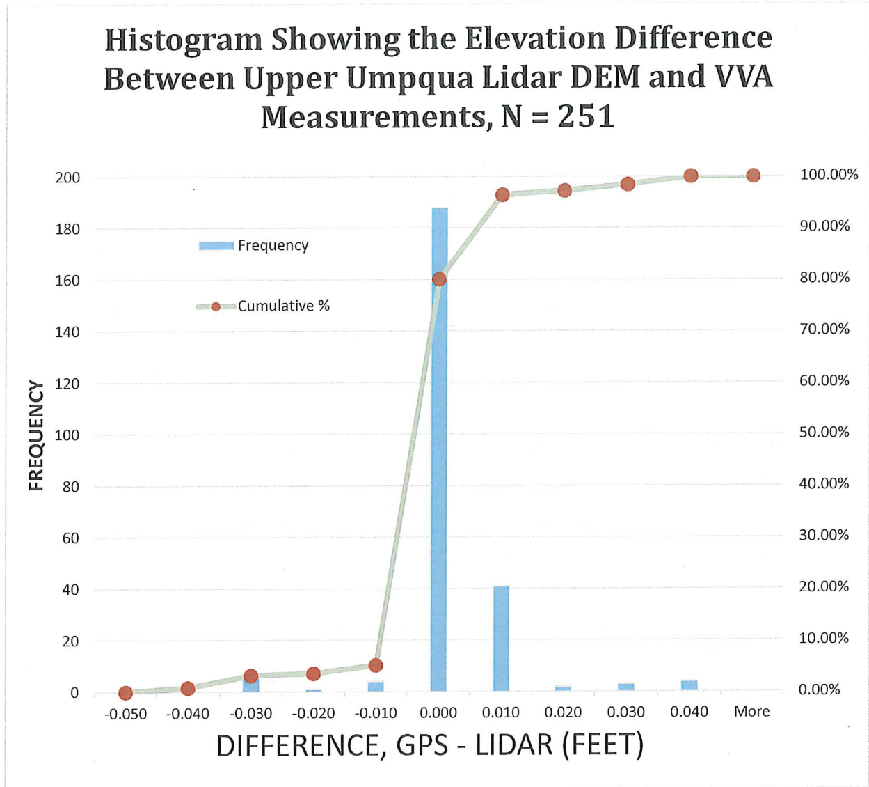
Figure 16. Histogram of VVA in feet.
