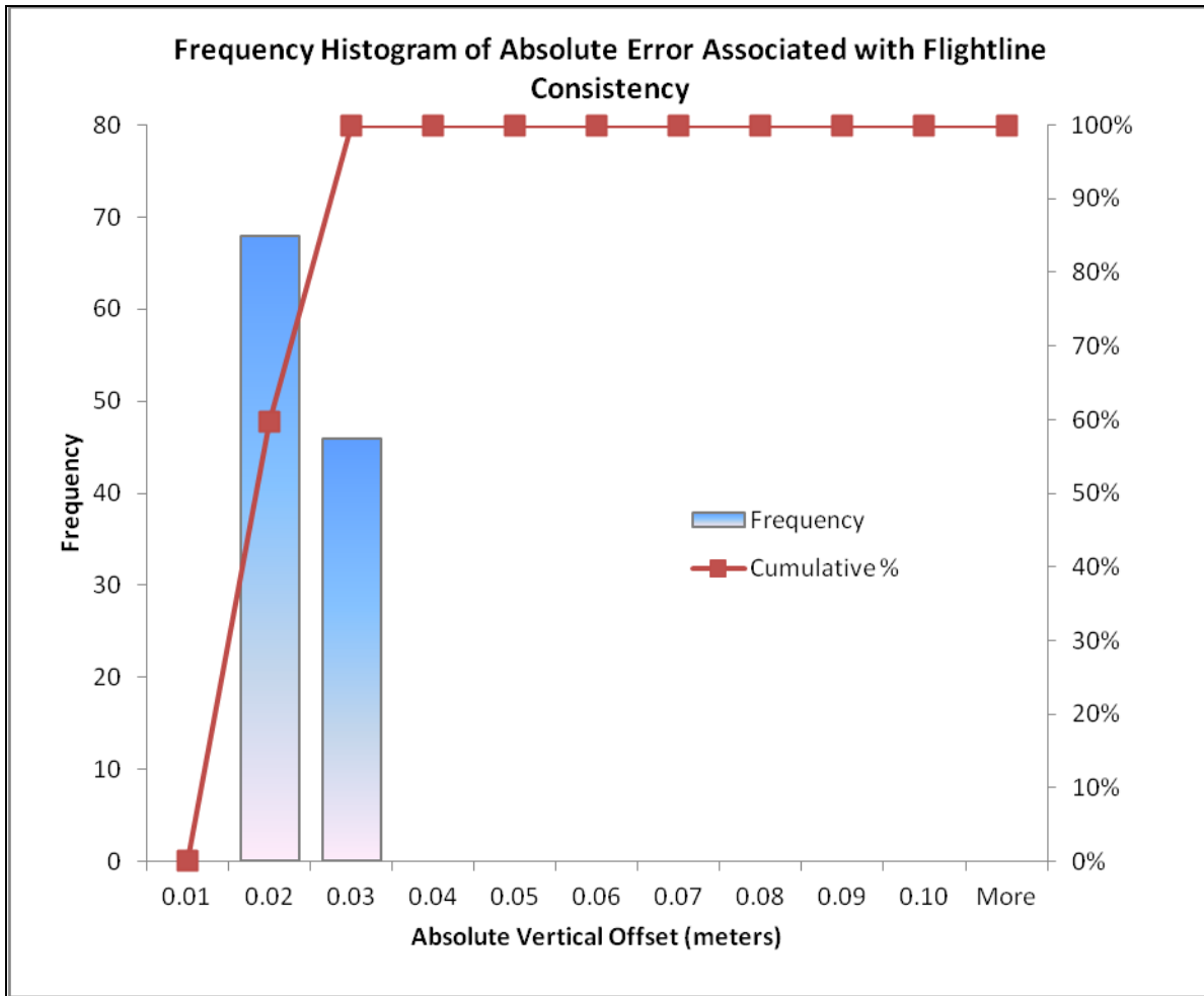
Figure 2. Calibration results for West Metro lidar.
