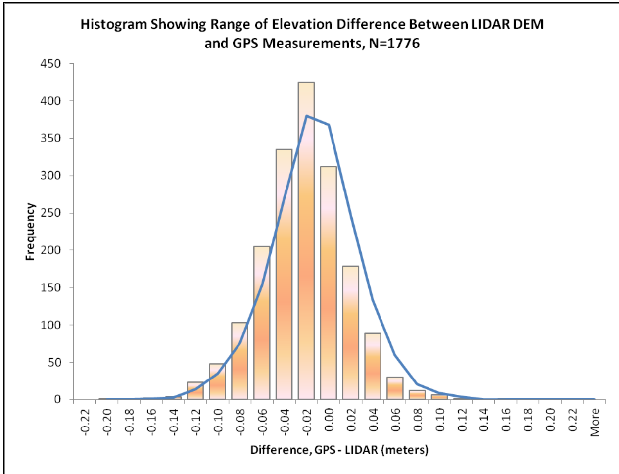
Figure 7. Histogram of absolute vertical accuracy
