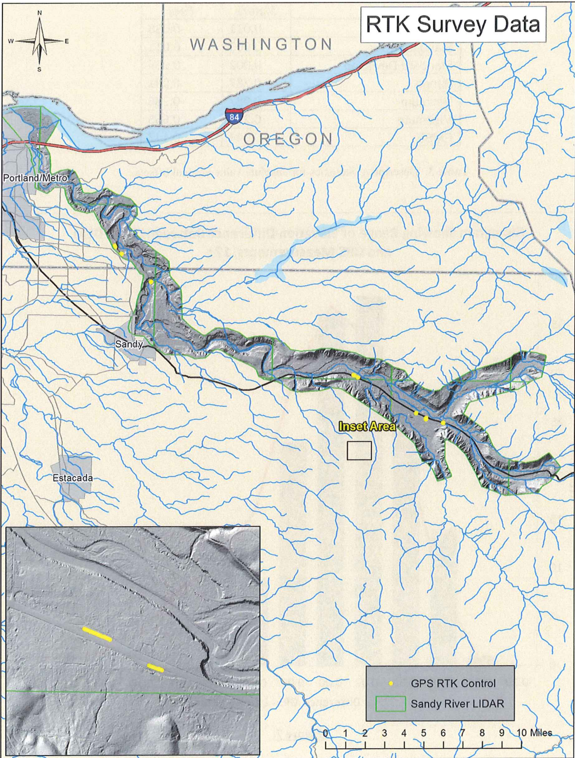
Figure 6. Locations of RTK control surveyed by DOGAMI. Data was used to test absolute accuracy for the Sandy River, OR lidar survey within the Delivery extent.
