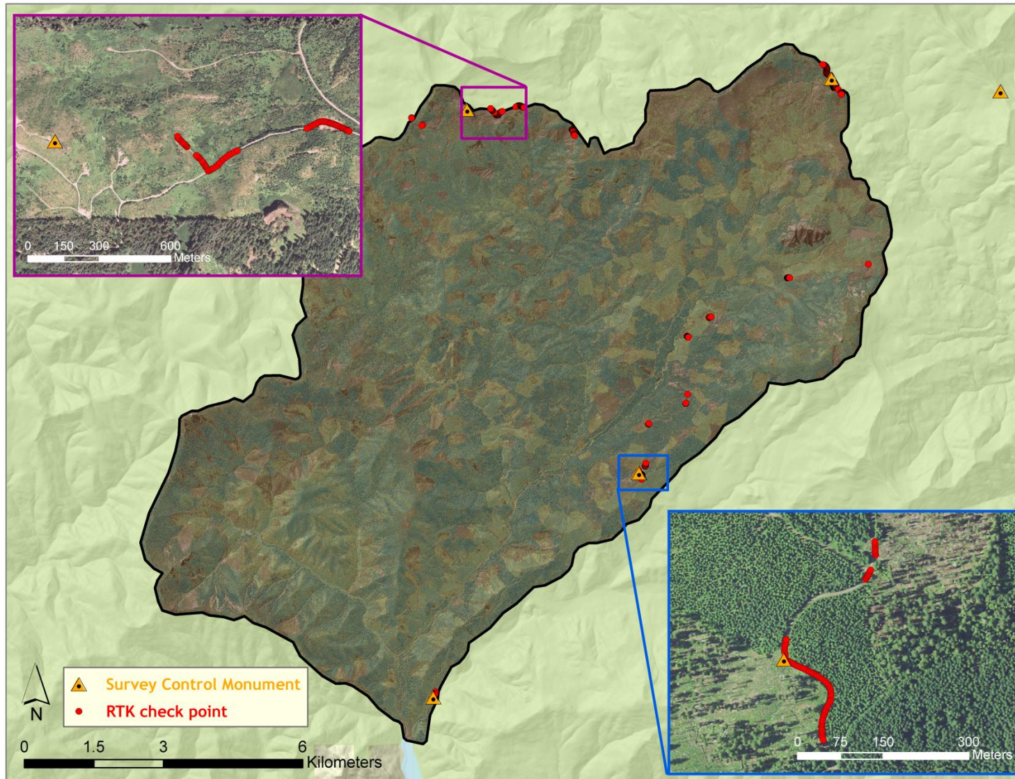
Figure 2. RTK check point and control monument locations used in the Blue River Watershed study areas
