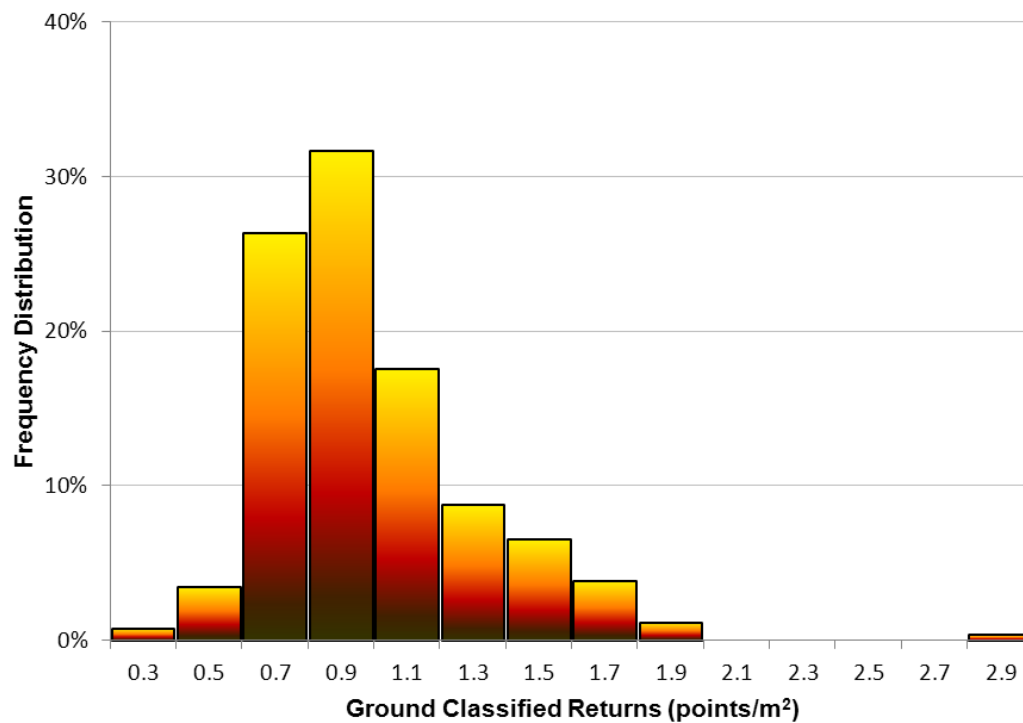
Figure 4. Density distribution for ground classified laser points in the Blue River Watershed and Big Springs SnoPark study areas.
