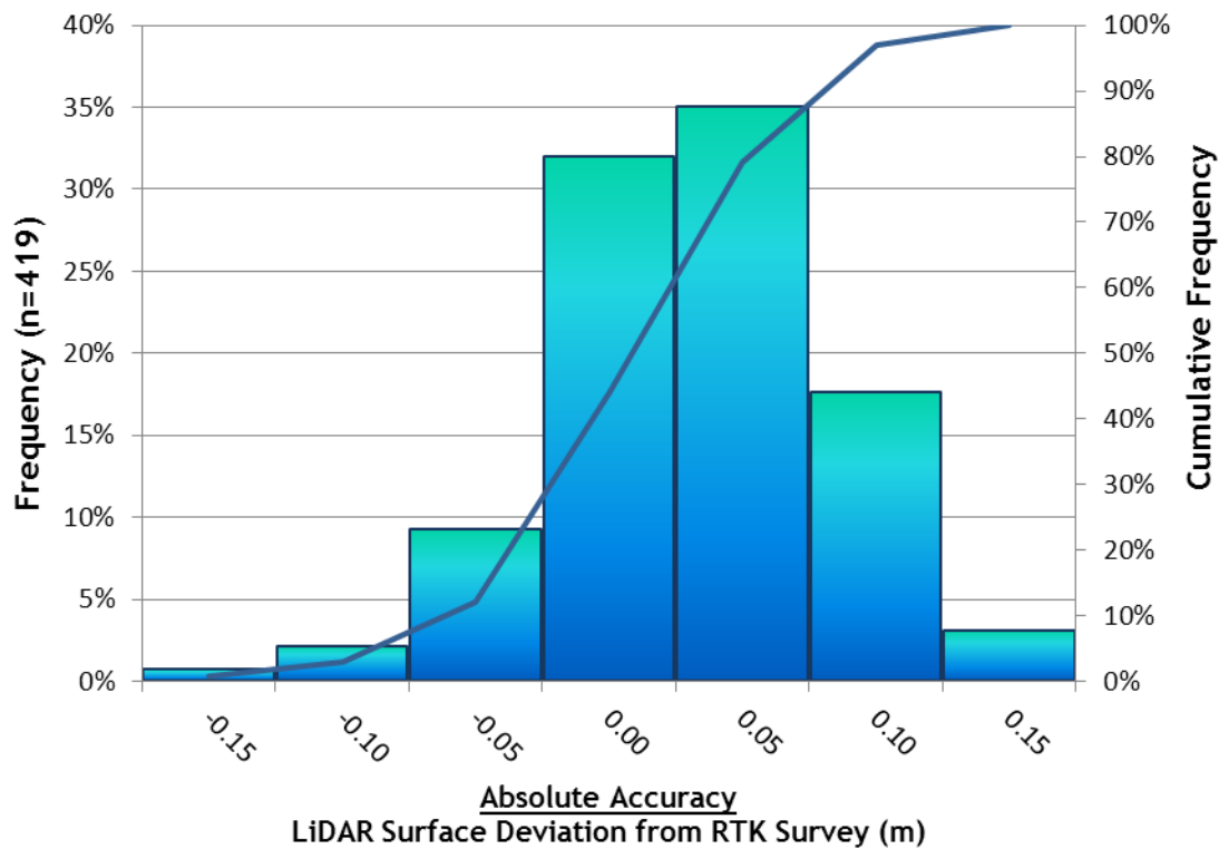
Figure 8. Absolute Accuracy - Histogram Statistics.
