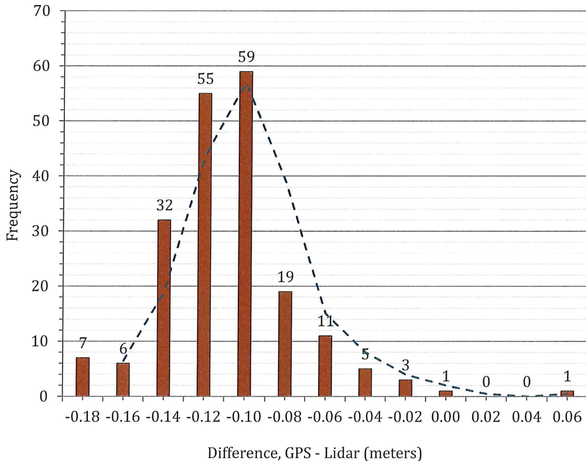
Range of Elevation Differences Between Lidar DEM and GPS Measurements
