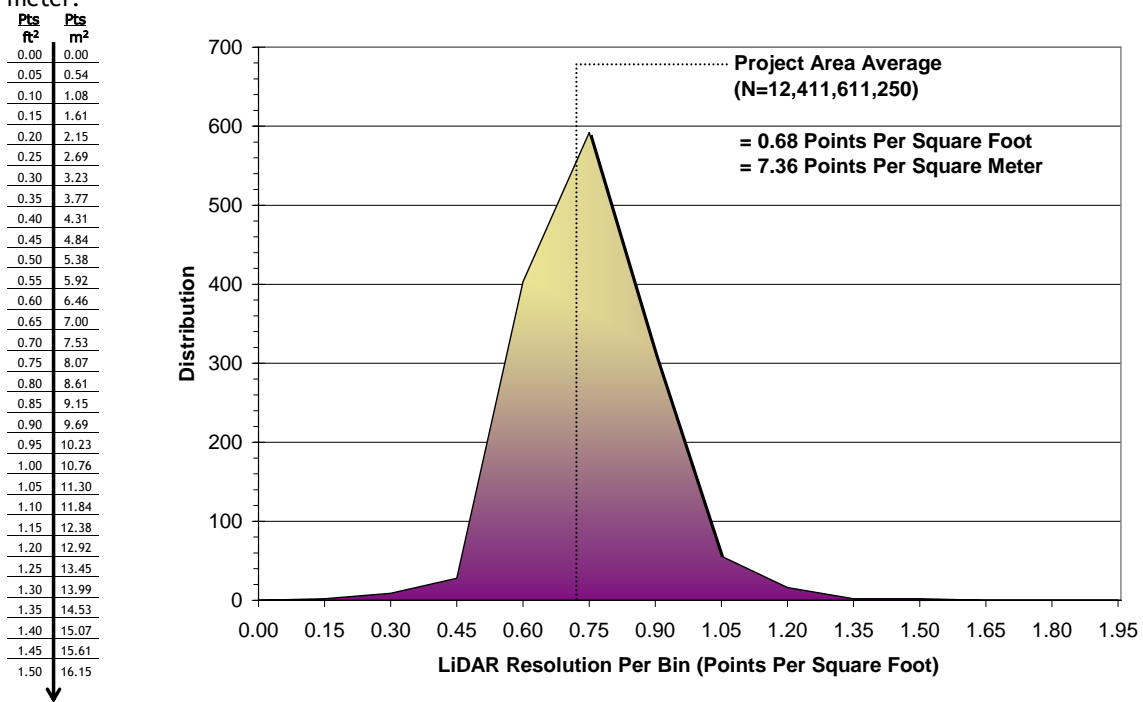
Figure 18. Image shows first return laser point data density in all Portland Area quads delivered to date, per 0.75' USGS Quad.
