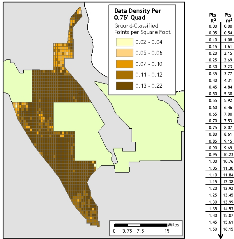
Figure 22. Image shows ground-classified laser point data density in all Portland Area quads delivered to date, per 0.75' USGS Quad.
