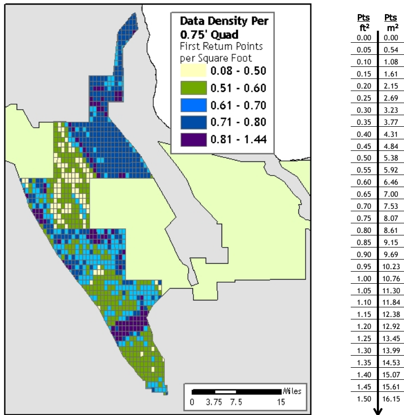
Figure 18. Image shows first return laser point data density in all Portland Area quads delivered to date, per 0.75' USGS Quad.
