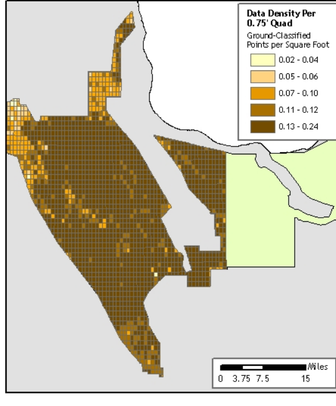
Figure 24. Image shows ground-classified laser point data density in all Portland Area quads delivered to date, per 0.75' USGS Quad.
