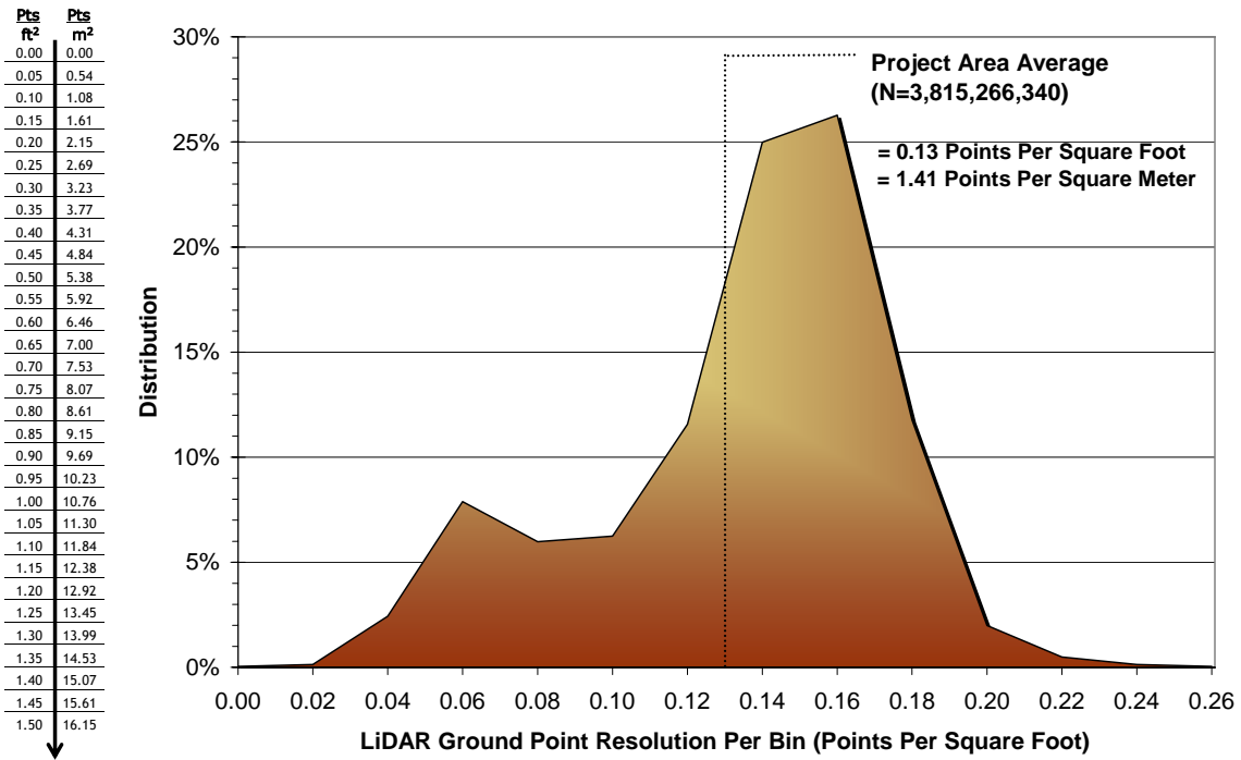
Figure 24. Image shows ground-classified laser point data density in all Portland Area quads delivered to date, per 0.75' USGS Quad.
