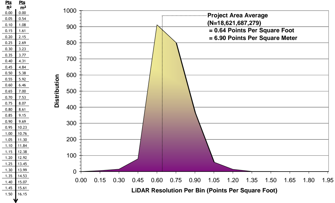
Figure 20. Image shows first return laser point data density in all Portland Area quads delivered to date, per 0.75' USGS Quad.
