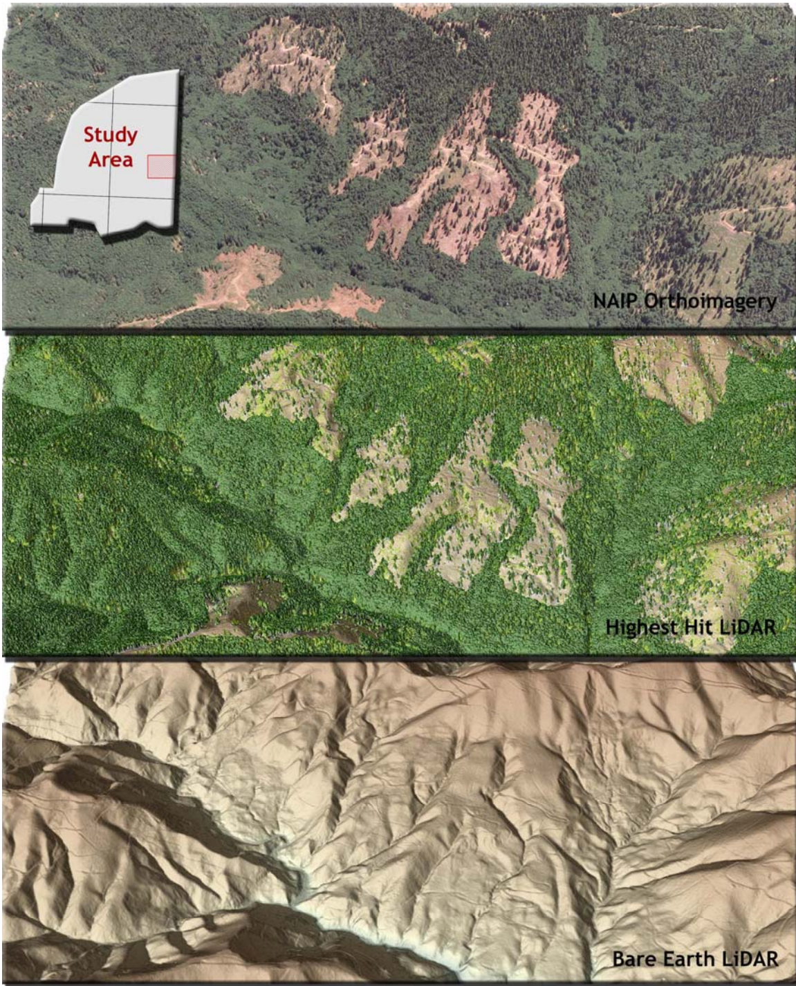
Figure 36. 3-d oblique view of LiDAR-derived surfaces in 7.5' Quad 45123E6, showing the upper portion of the Little North Fork Wilson River watershed in the ODF South study area.
