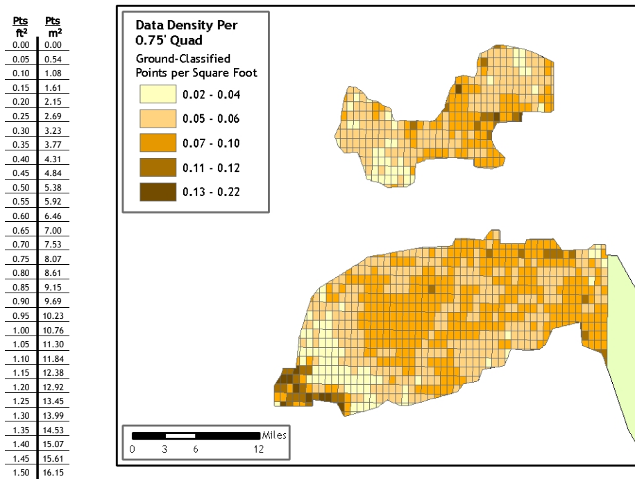
Figure 22. Image shows ground-classified laser point data density per 0.75' USGS Quad in both ODF's AOIs.
