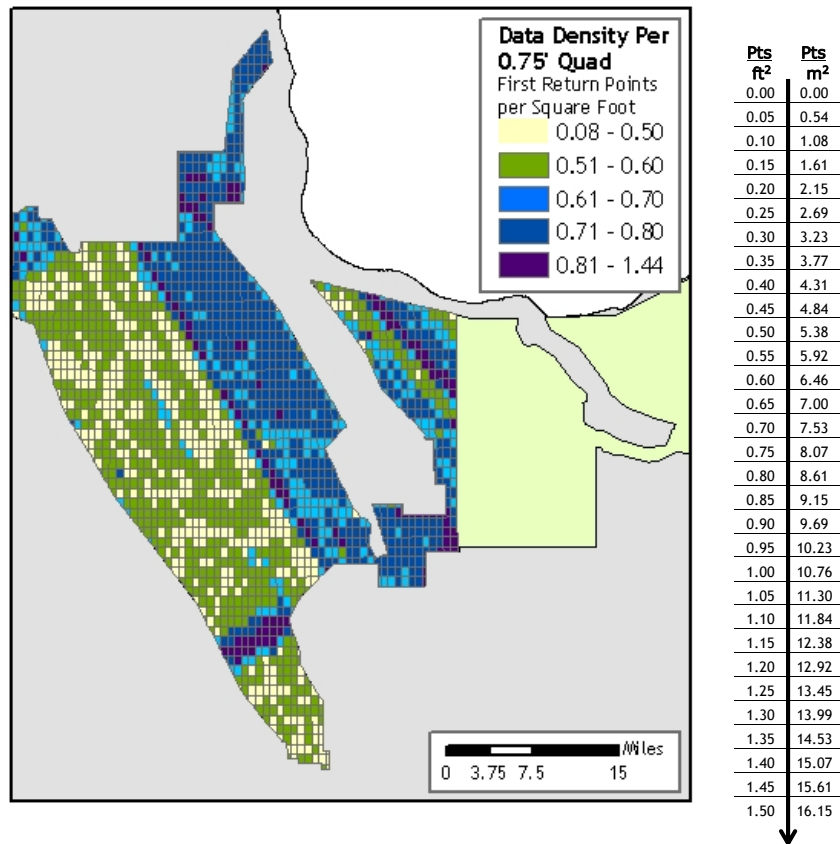
Figure 20. Image shows first return laser point data density in all Portland Area quads delivered to date, per 0.75' USGS Quad.
