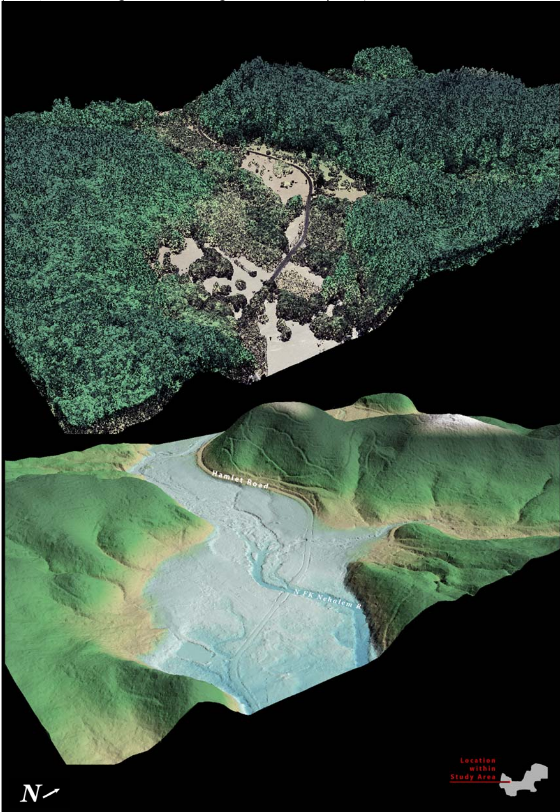
Figure 26. 3-d oblique view of LiDAR-derived surfaces in Quad 45123G6115, showing the North Fork Nehalem River and Hamlet Road in the ODF North Study Area (top image derived from all points, bottom image derived from ground-classified points).
