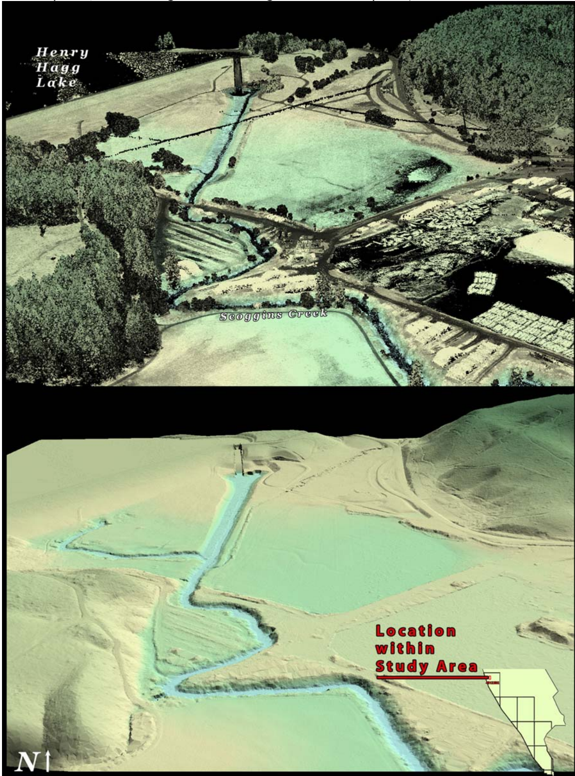
Figure 32. 3-d oblique view of LiDAR-derived surfaces in 0.75' Quad 45123D2109-110,114-115, showing Henry Hagg Lake and Scoggins Creek in the DOGAMI study area (top image derived from all points, bottom image derived from ground-classified points).
