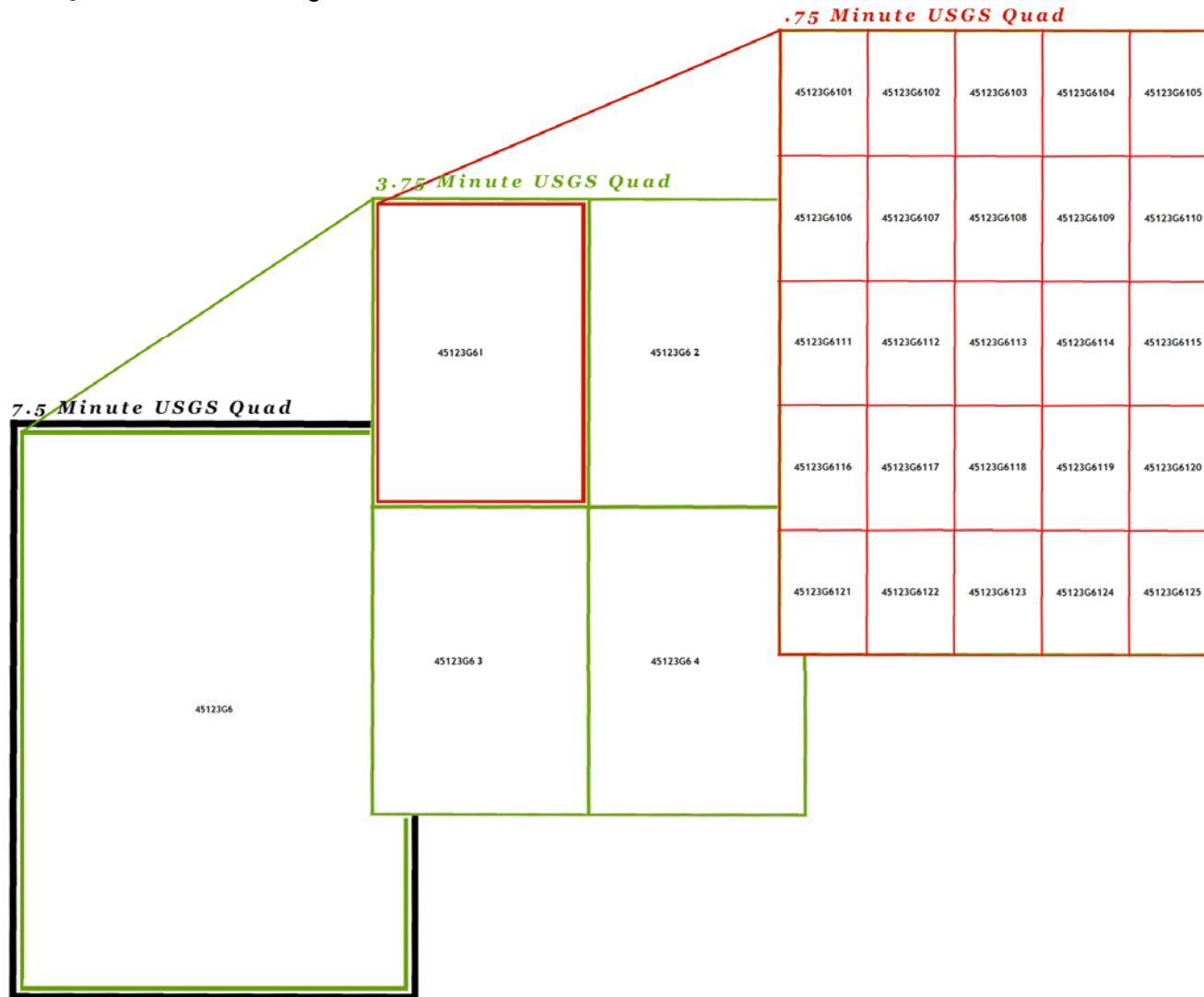
Figure 25. 0.75' USGS Quad Delineation Naming Convention
