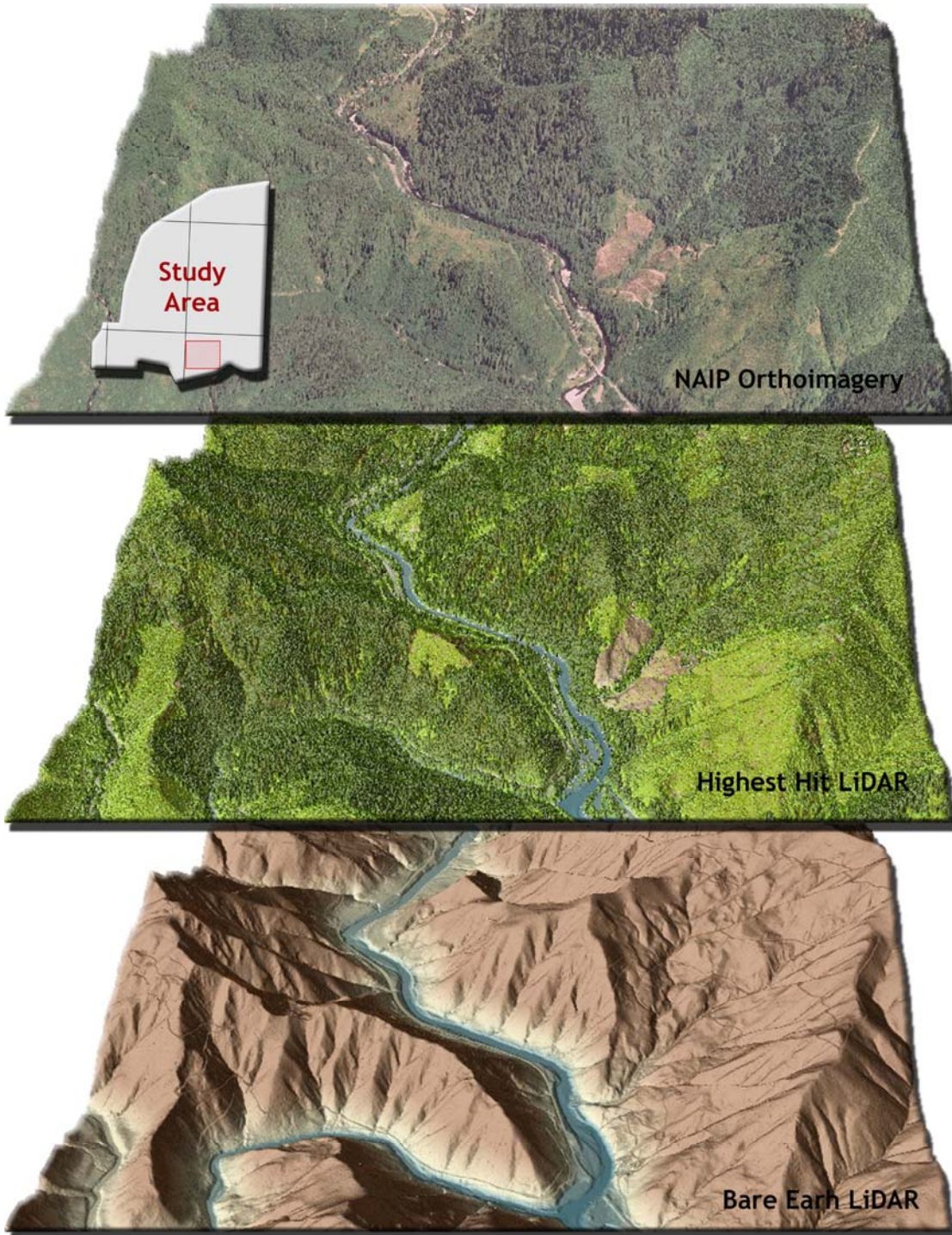
Figure 34. 3-d oblique view of LiDAR-derived surfaces in 7.5' Quad 45123D6, showing Wilson River near the Little North Fork confluence in the ODF South study area.
