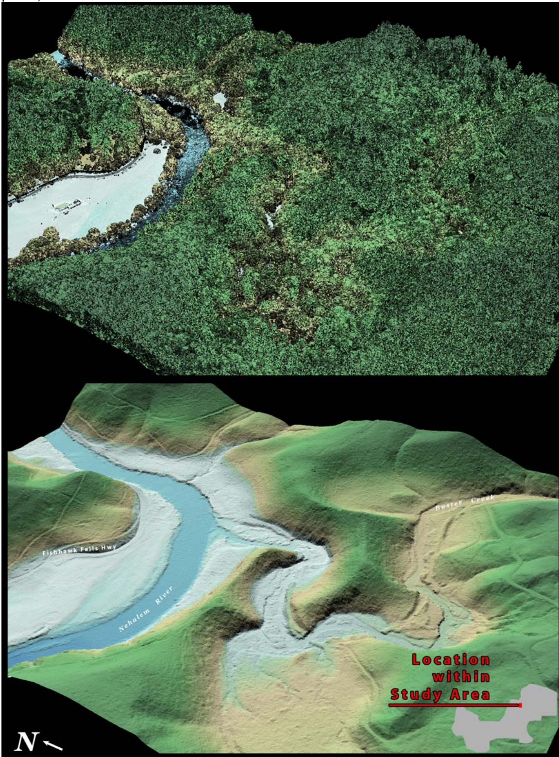
Figure 28. 3-d oblique view of LiDAR-derived surfaces in Quad 45123G6414, showing the confluence of Buster Creek with the Nehalem River, and Fishhawk Falls Road in the ODF North Study Area. (Top image derived from all points, bottom image derived from ground-classified points).
