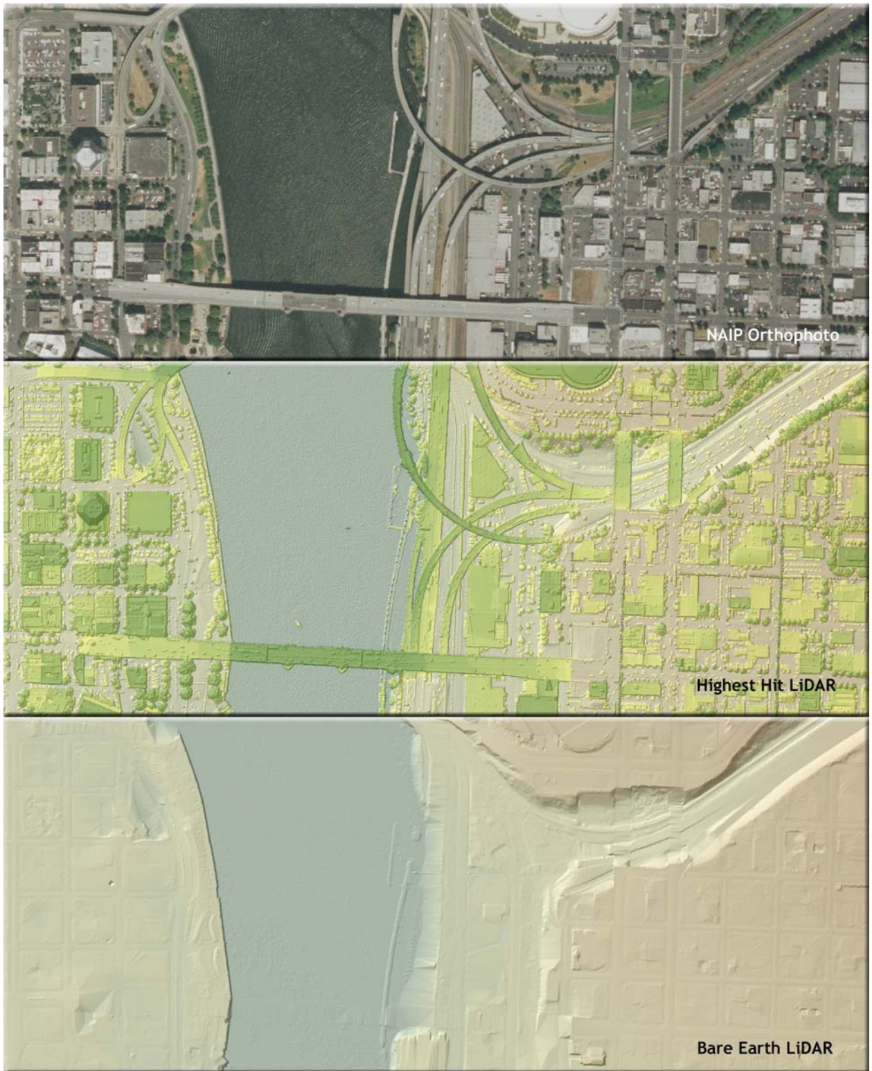
Figure 49. 3-d oblique view of the I-5 and I-84 interchange near downtown Portland.
