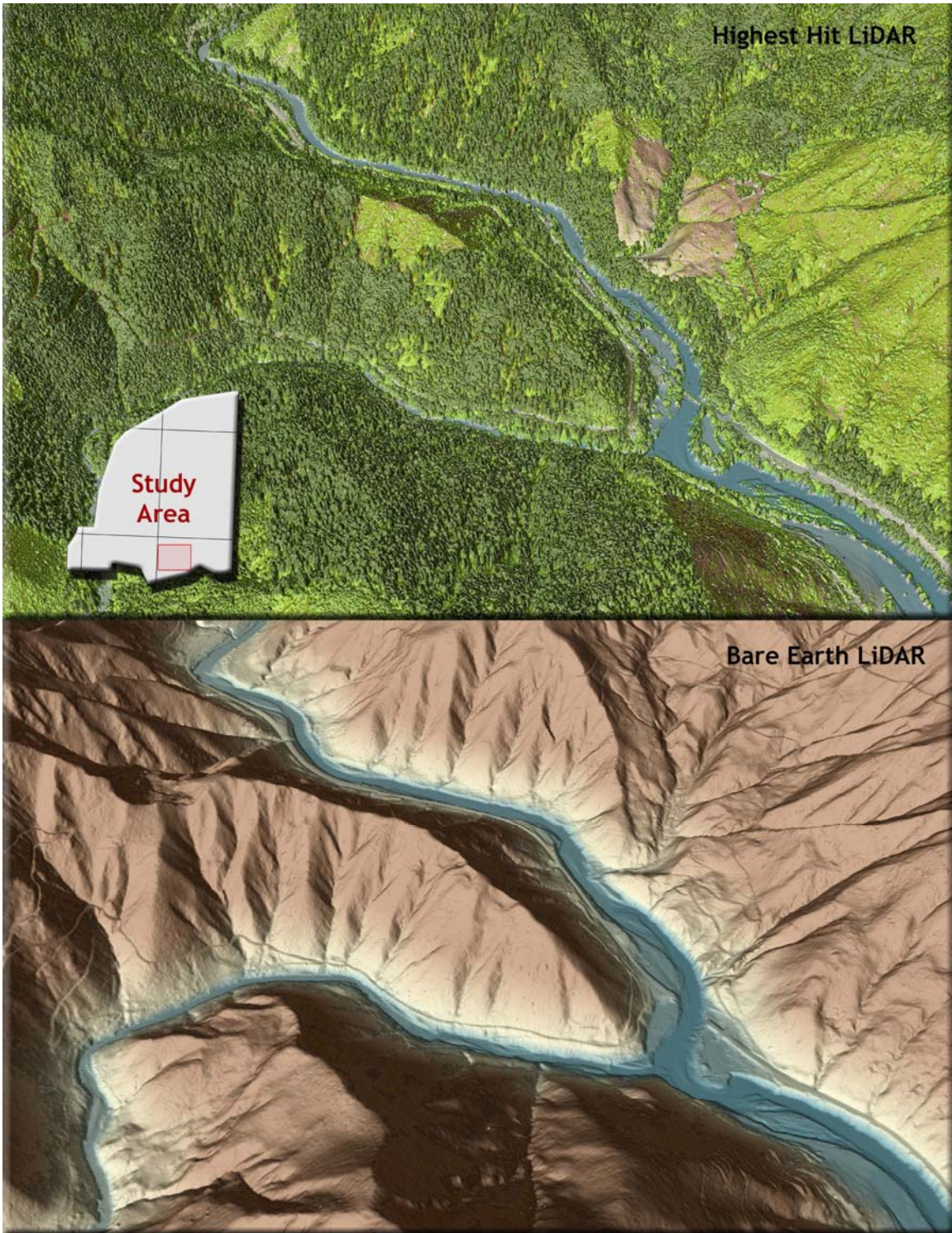
Figure 35. 3-d oblique view of LiDAR-derived surfaces in 7.5' Quad 45123D6, showing the confluence of the Wilson and Little North Fork Rivers in the ODF South study area.
