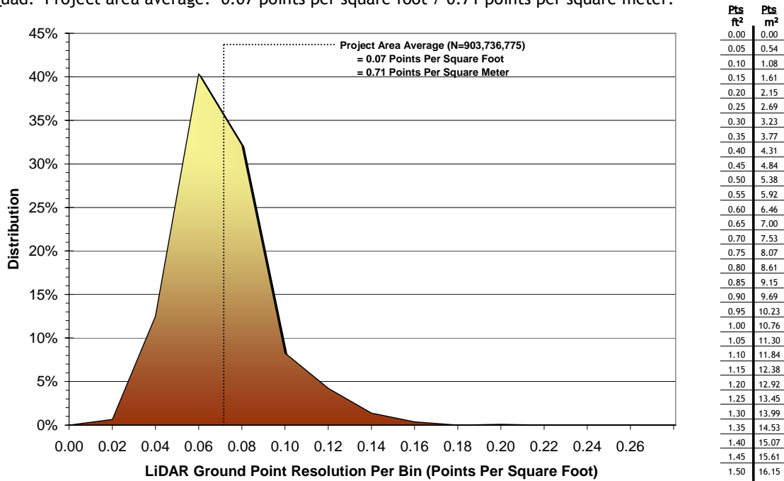
Figure 22. Image shows ground-classified laser point data density per 0.75' USGS Quad in both ODF's AOIs.
