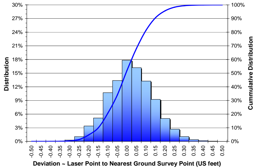
Figure 16. Study Area: Point Absolute Deviation Statistics
