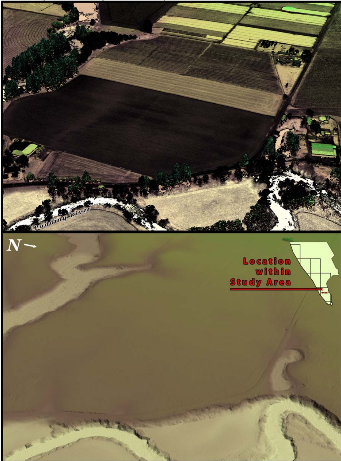
Figure 30. 3-d oblique view of LiDAR-derived surfaces in 0.75' Quad 45122A7108, showing a short reach of the Pudding River in the DOGAMI study area (top image derived from all points, bottom image derived from ground-classified points).
