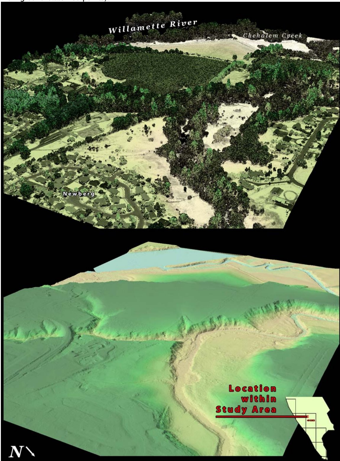
Figure 31. 3-d oblique view of LiDAR-derived surfaces in 0.75' Quad 45122C8307-308,312-313, showing the confluence of Chehalem Creek and the Willamette River, near the southwest edge of Newberg in the DOGAMI study area (top image derived from all points, bottom image derived from ground-classified points).
