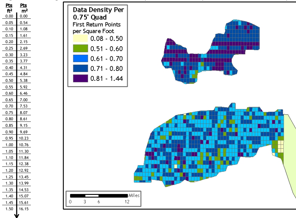
Figure 18. Image shows first return laser point data density in both of ODF's AOIs, per 0.75' USGS Quad.
