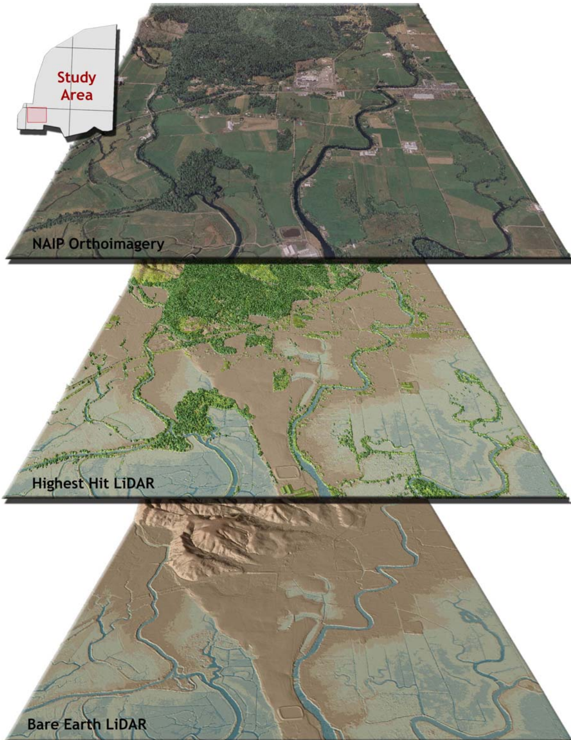
Figure 33. 3-d oblique view of LiDAR-derived surfaces in 7.5' Quad 45123D7, showing Kilchis and Wilson Rivers in the ODF South study area.
