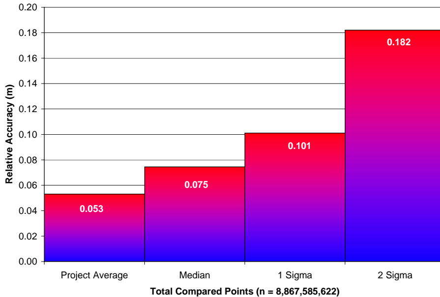
Figure 14. Statistical relative accuracies, non slope-adjusted.
