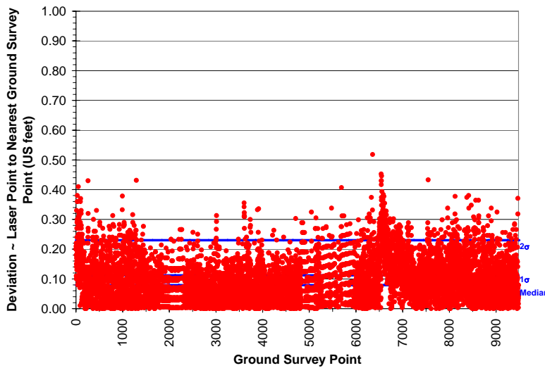
Figure 16. Study Area: Point Absolute Deviation Statistics
