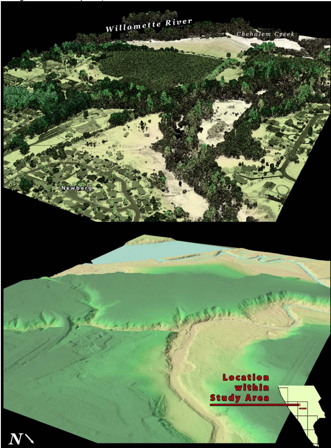
Figure 6.6. 3-d oblique view of LiDAR-derived surfaces in 0.75' Quad 45122C8307-308,312-313, showing the confluence of Chehalem Creek and the Willamette River, near the southwest edge of Newberg in the DOGAMI study area (top image derived from all points, bottom image derived from ground-classified points).
