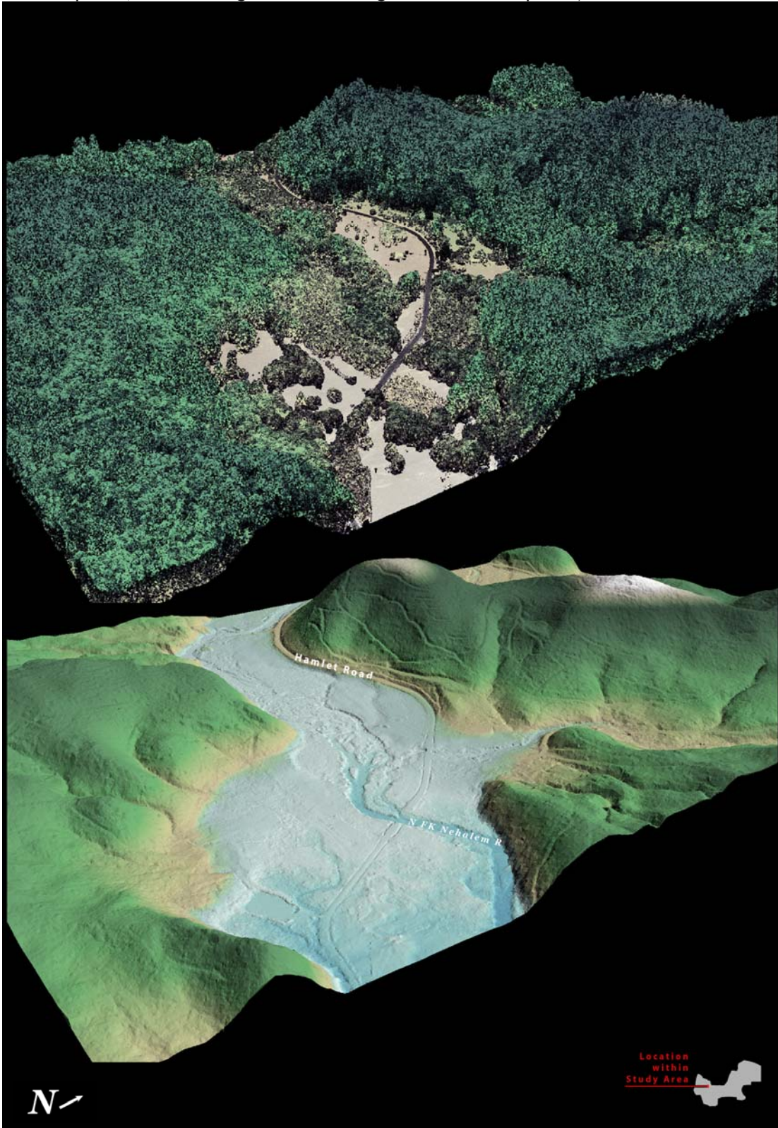
Figure 6.1. 3-d oblique view of LiDAR-derived surfaces in Quad 45123G6115, showing the North Fork Nehalem River and Hamlet Road in the ODF North Study Area (top image derived from all points, bottom image derived from ground-classified points).
