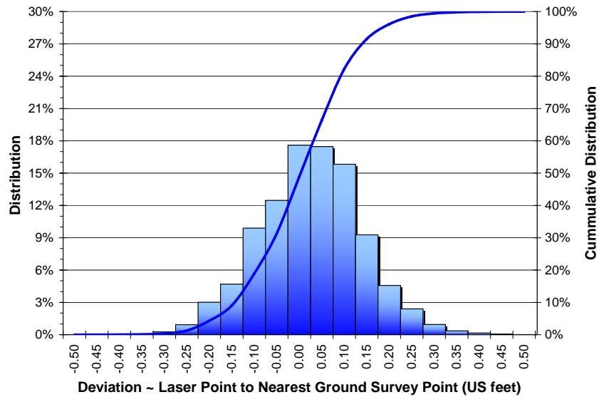
Figure 4.4. Study Area: Point Absolute Deviation Statistics
