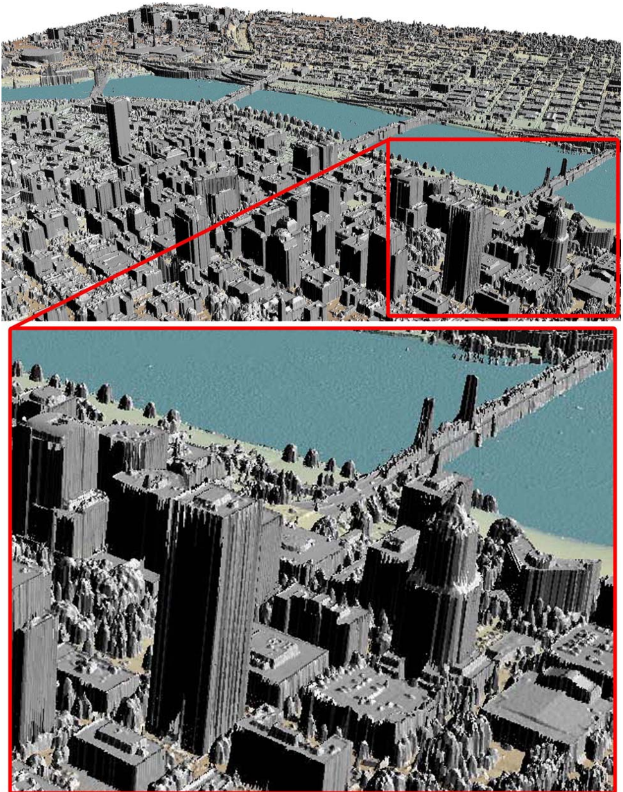
Figure 6.19. 3-d oblique view of LiDAR-derived images showing the highest hit surface of downtown Portland, looking eastward.
