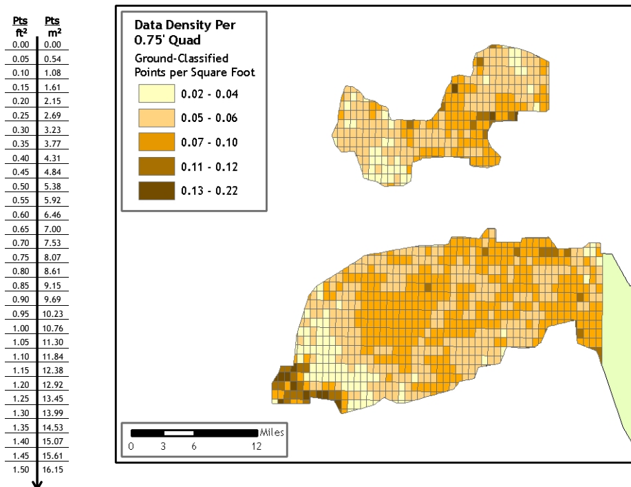
Figure 4.10. Image shows ground-classified laser point data density per 0.75' USGS Quad in both ODF's AOIs.
