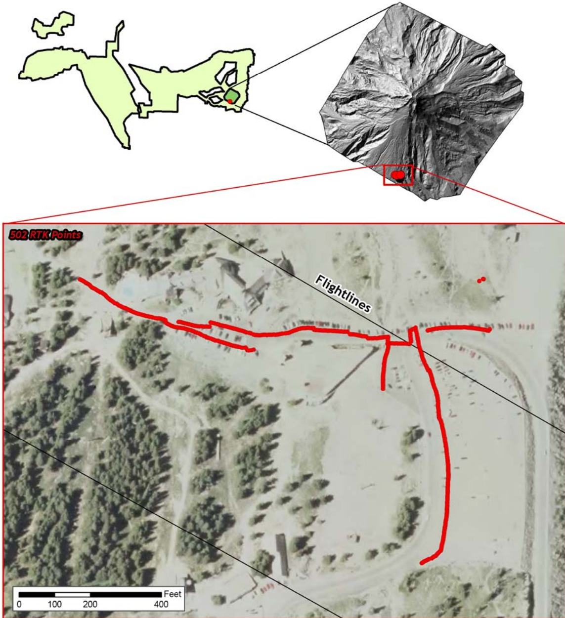
Figure 2.12. RTK point locations in the DOGAMI study areas; color images are NAIP Orthoimages; RTK points shown over bare-earth surface created from LiDAR data.
