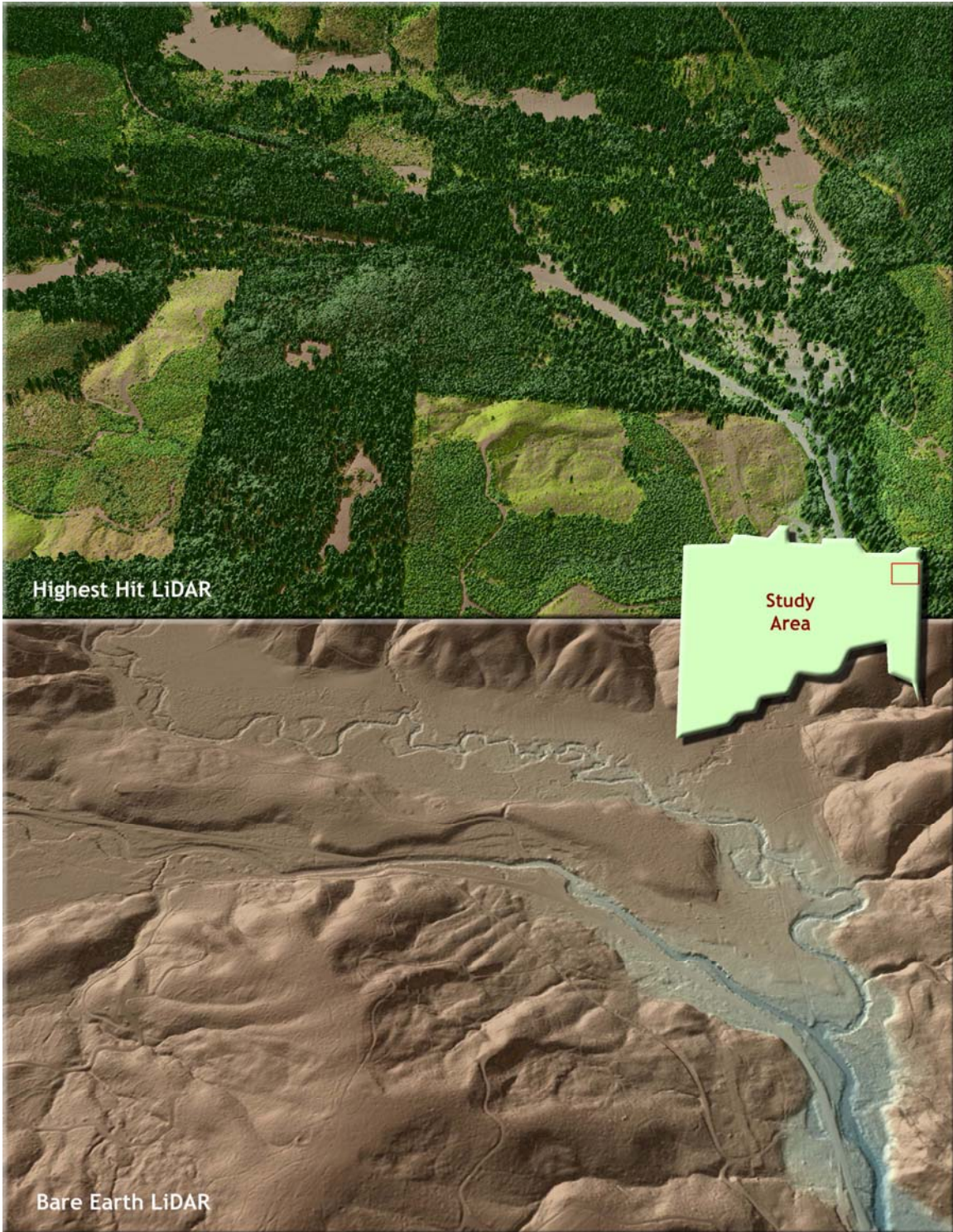
Figure 6.16. 3-d oblique view of LiDAR-derived surfaces looking north across confluence of Gales Creek and Beaver Creek.
