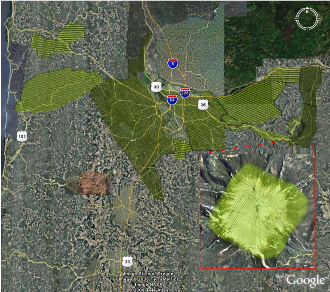
Figure 2.1. Planned flight lines for the DOGAMI AOIs illustrated over oblique 3-D GoogleEarth images, showing flightline locations, swath width, and overlap between flight lines.
