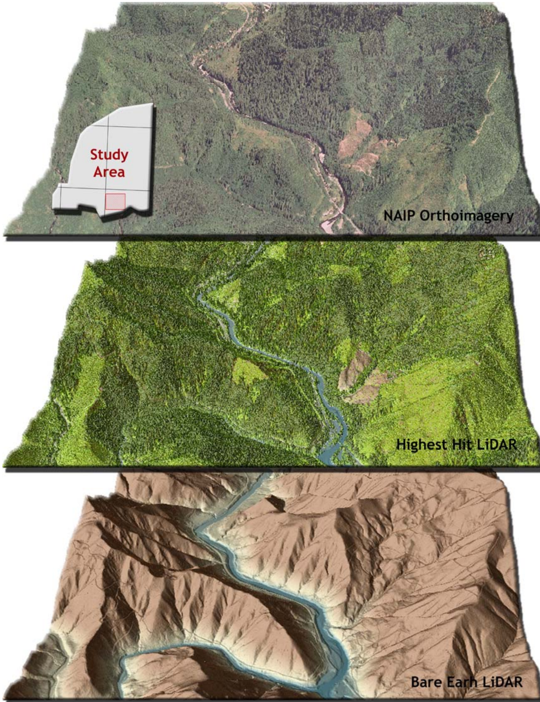
Figure 6.9. 3-d oblique view of LiDAR-derived surfaces in 7.5' Quad 45123D6, showing Wilson River near the Little North Fork confluence in the ODF South study area.
