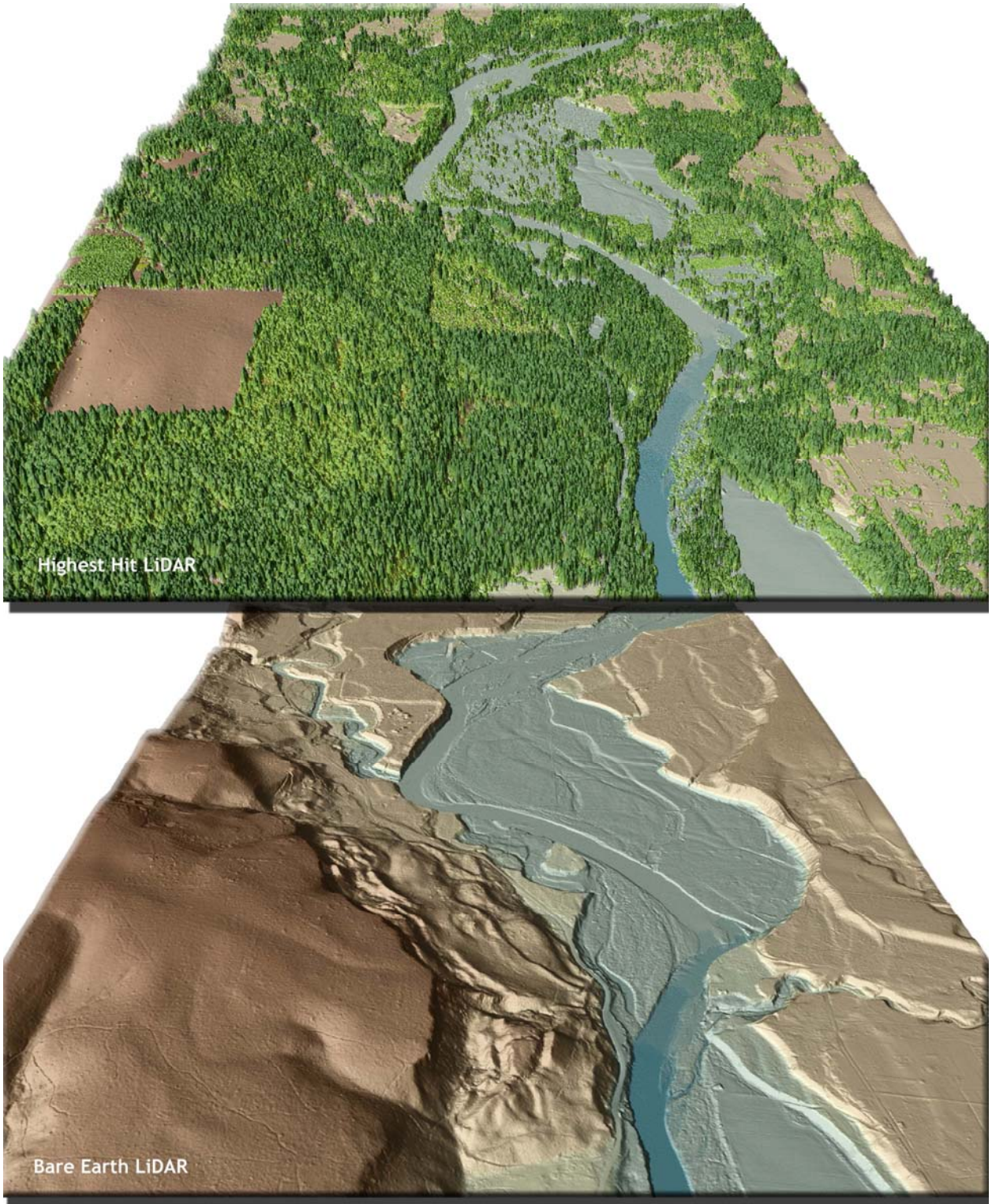
Figure 6.29. 3-d oblique view of the Clackamas River (looking upstream) near Foster Creek (entering from lower right of image) and Deep Creek (entering from upper left of image).
