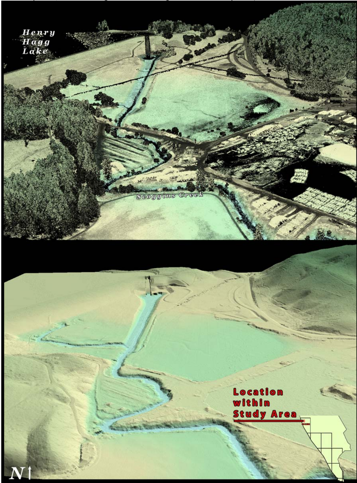
Figure 6.7. 3-d oblique view of LiDAR-derived surfaces in 0.75' Quad 45123D2109-110,114-115, showing Henry Hagg Lake and Scoggins Creek in the DOGAMI study area (top image derived from all points, bottom image derived from ground-classified points).
