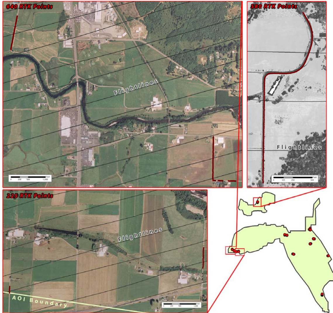
Figure 2.4. RTK point locations in the ODF study areas; color images are NAIP Orthoimages, black and white image is 1.5-foot resolution intensity image derived from LiDAR data.
