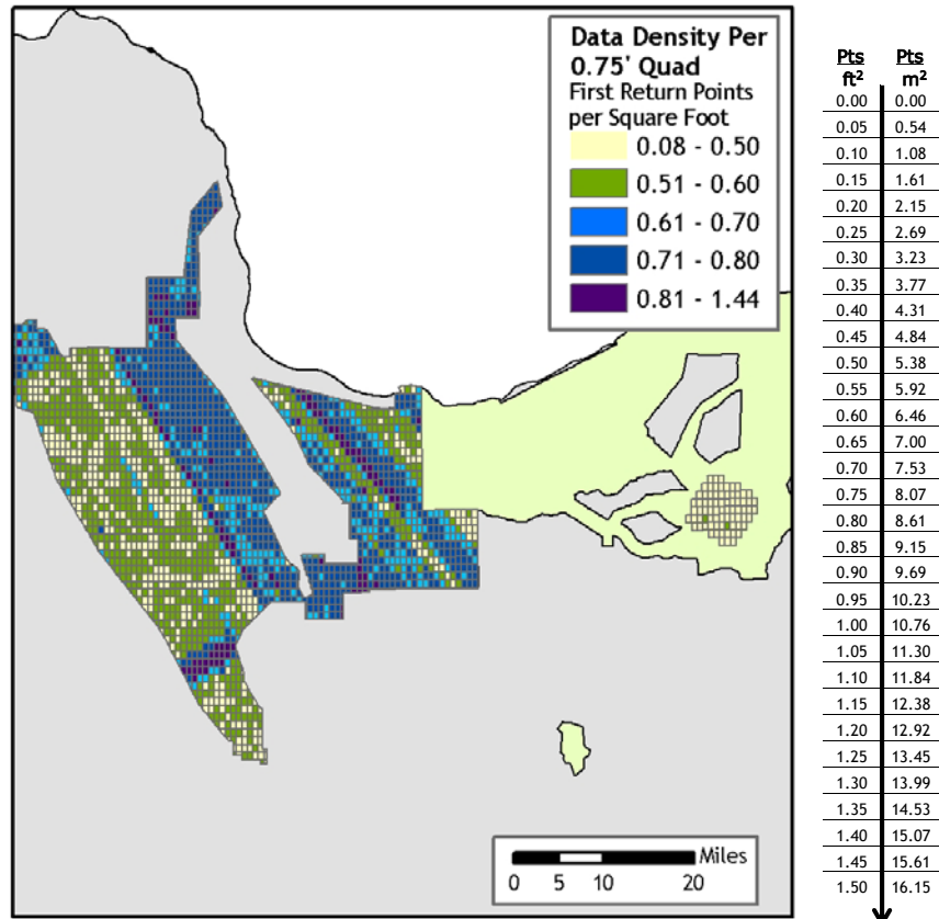
Figure 4.8. Image shows first return laser point data density in all Portland Area quads delivered to date, per 0.75' USGS Quad.
