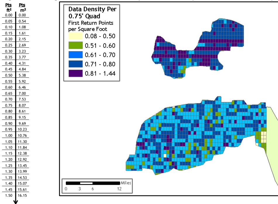
Figure 4.6. Image shows first return laser point data density in both of ODF's AOIs, per 0.75' USGS Quad.
