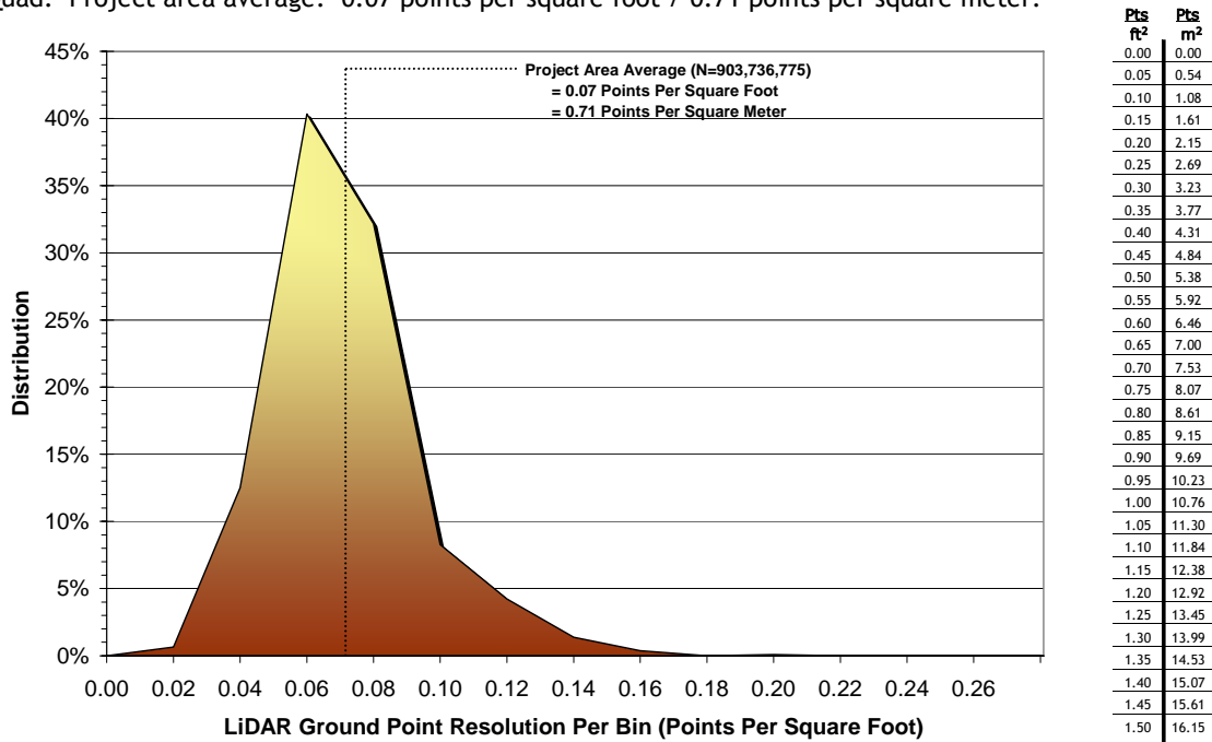
Figure 4.10. Image shows ground-classified laser point data density per 0.75' USGS Quad in both ODF's AOIs.
