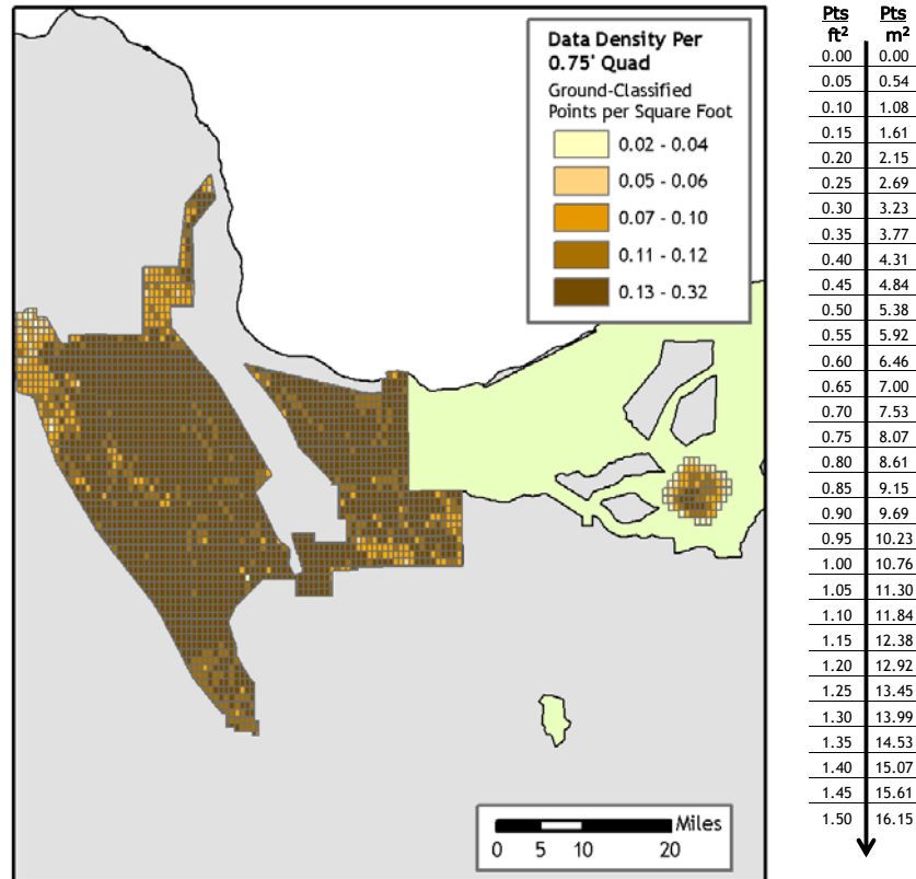
Figure 4.12. Image shows ground-classified laser point data density in all Portland Area quads delivered to date, per 0.75' USGS Quad.
