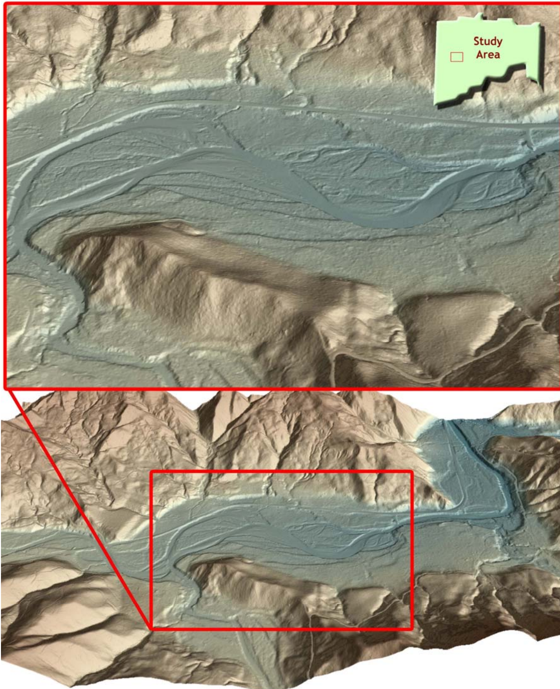
Figure 6.14. 3-d oblique view of LiDAR-derived surfaces looking south over the Wilson River near the North Fork confluence.
