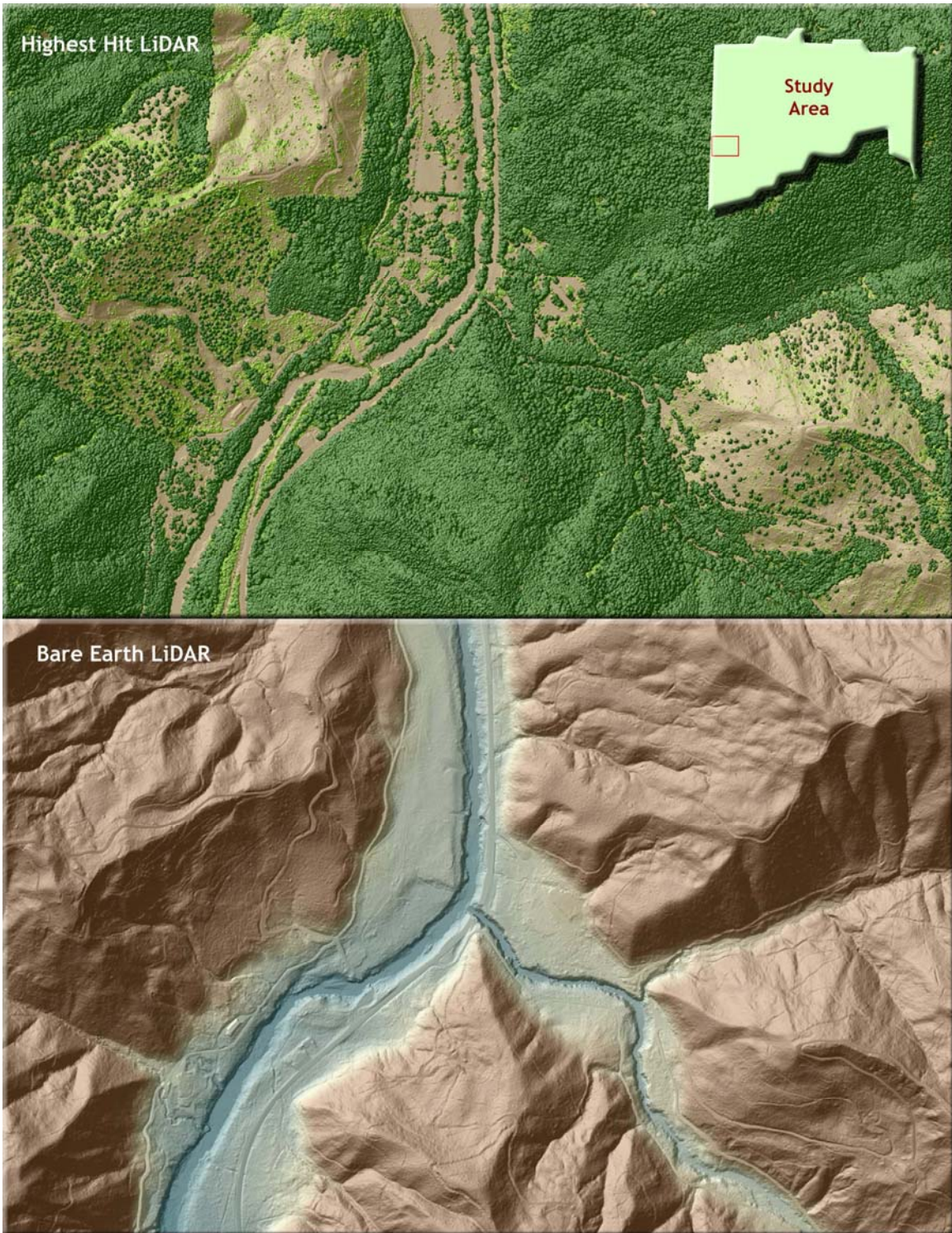
Figure 6.17. 3-d oblique view of LiDAR-derived surfaces showing the Wilson River at the Jordan Creek confluence.
