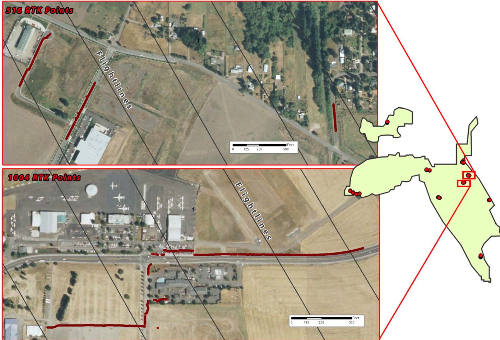
Figure 2.6. RTK point locations in the DOGAMI study areas; color images are NAIP Orthoimages.
