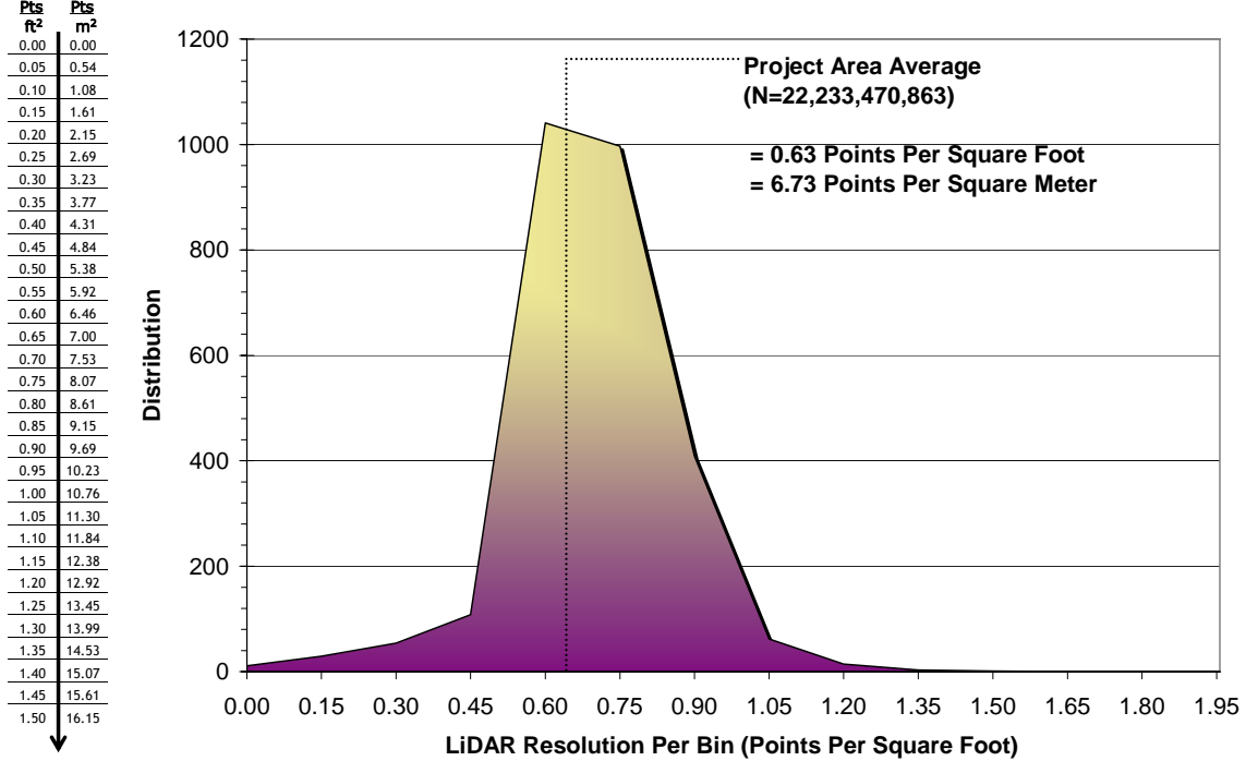
Figure 4.7. Histogram of first return laser point data density in all Portland Area quads delivered to date, per 0.75' USGS Quad. Project area average: 0.63 points per square foot / 6.73 points per square meter.
