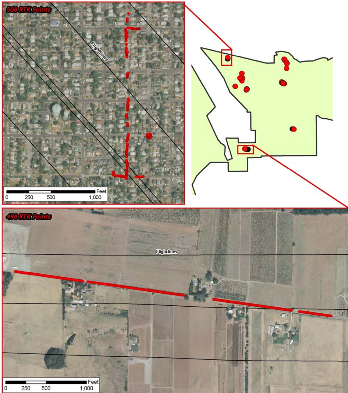
Figure 2.8. RTK point locations in the DOGAMI study areas; color images are NAIP Orthoimages.
