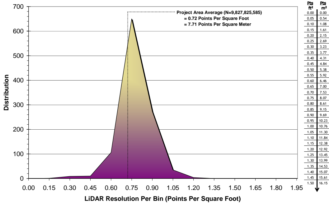
Figure 4.5. Histogram of first return laser point data density in both of ODF's AOIs, per 0.75' USGS Quad. Project area average: 0.72 points per square foot / 7.71 points per square meter.
