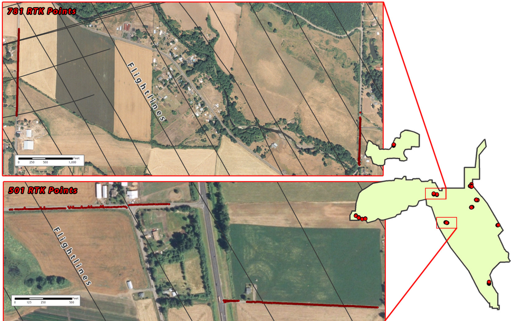
Figure 2.5. RTK point locations in the DOGAMI study areas; color images are NAIP Orthoimages.
