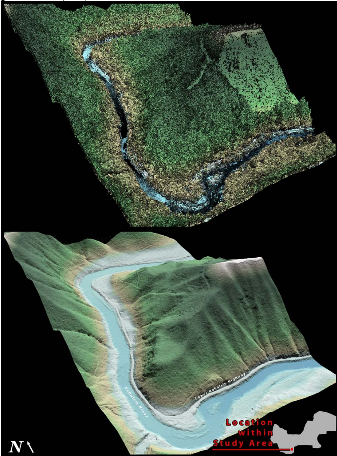
Figure 6.2. 3-d oblique view of LiDAR-derived surfaces in Quad 45123G6414, showing the Nehalem River and the Lower Nehalem Highway, just inside the Clatsop State Forest boundary in the ODF North Study Area. (Top image derived from all points, bottom image derived from ground-classified points).
