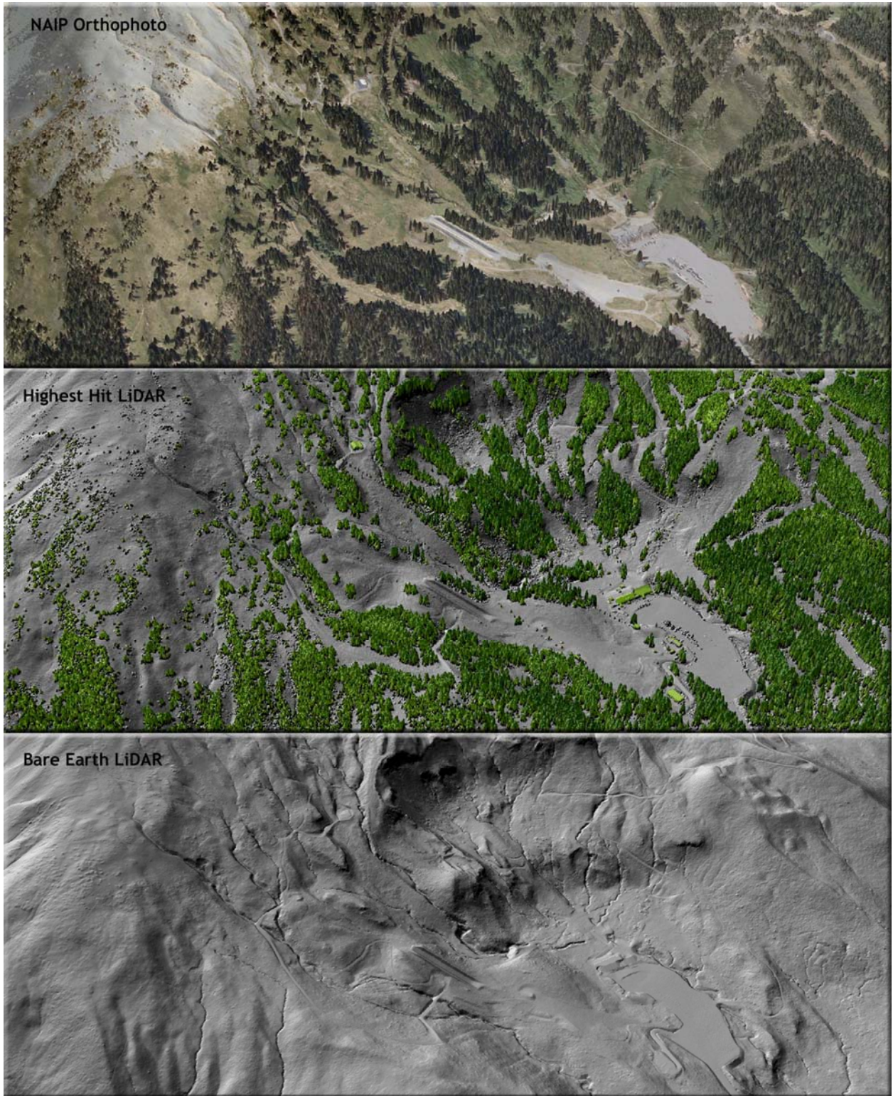
Figure 6.38. 3-d oblique view of Mount Hood Meadows ski area east of Timberline Lodge.
