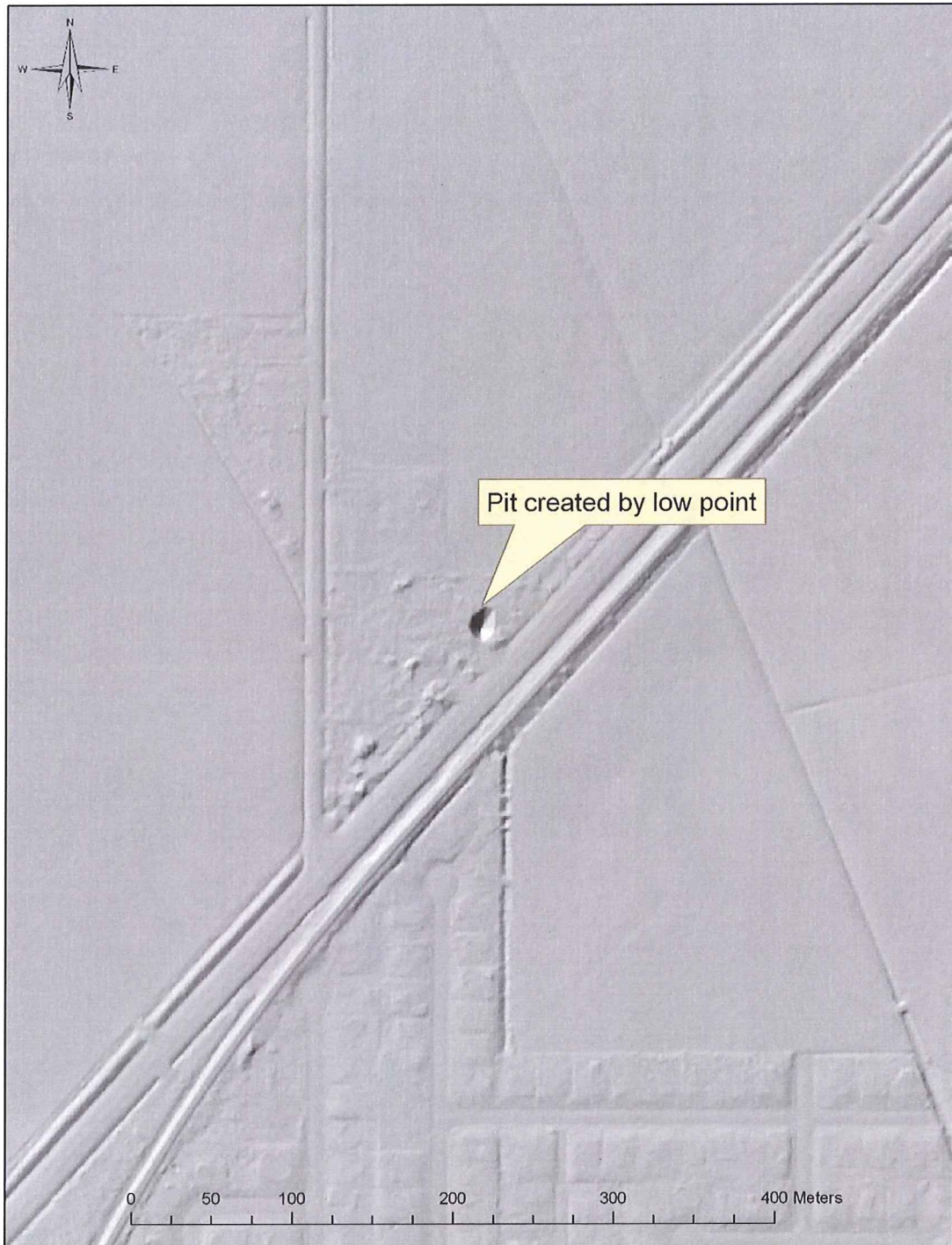
Figure 5. Example of “Pit” observable when comparing bare earth to highest hit models. Pits are caused when standing water absorbs the lidar pulse. Pits are evident in ground model as the lowest point elevation is assigned to the grid cell value. Inversely the pit is not observable in the highest hit model as the highest point elevation is assigned to the grid value
