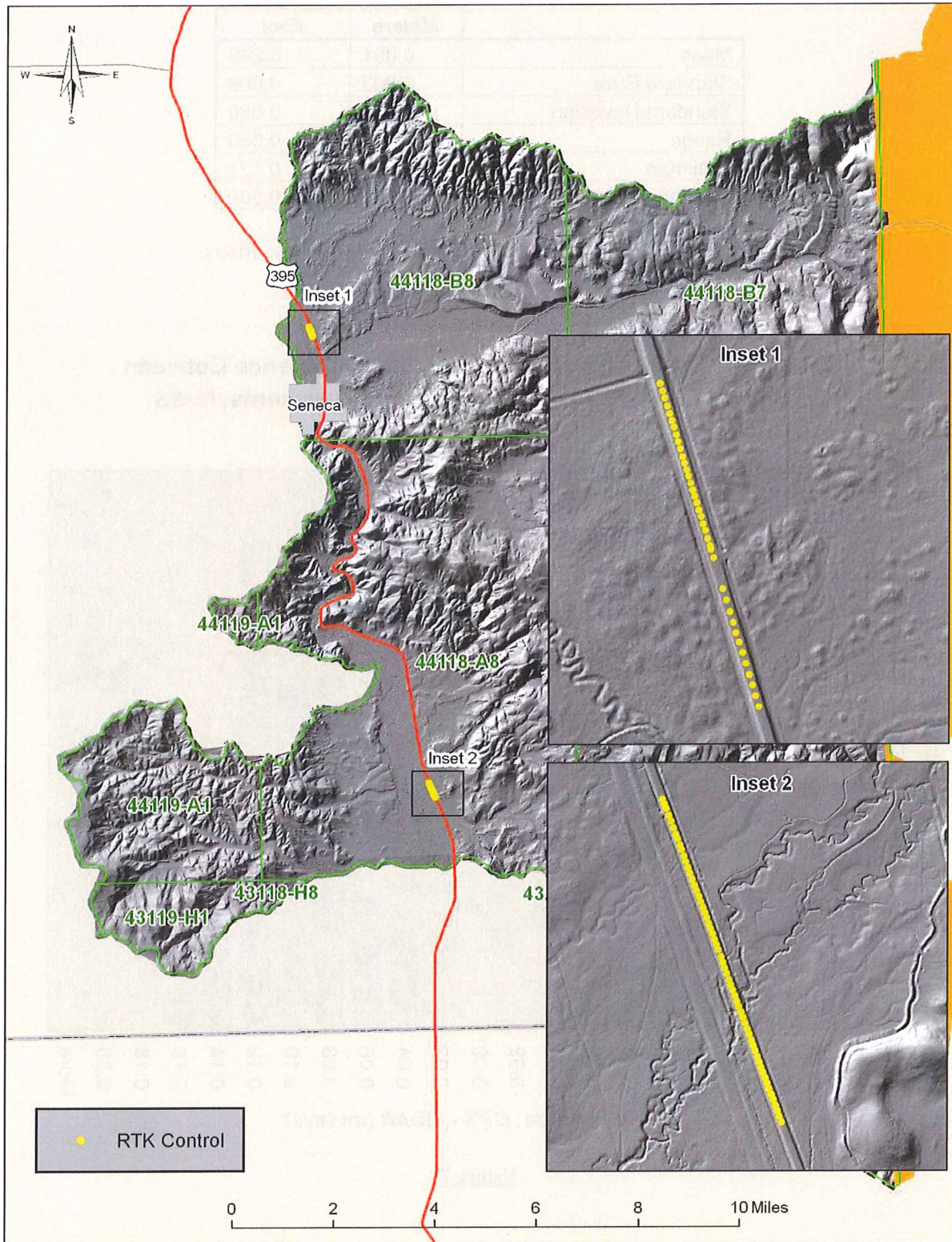
Figure 6. Locations of RTK control surveyed by DOGAMI. Data was used to test absolute accuracy for the Malheur lidar survey within the Delivery extent.
