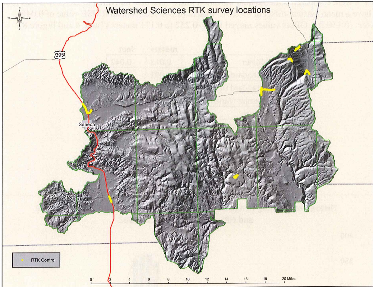
Figure 9. Watershed Sciences RTK survey locations
