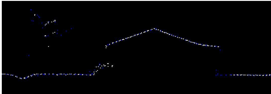
Figure 6. Profile of a lidar point cloud cross section of buildings. Points are colorized by flight line number.
